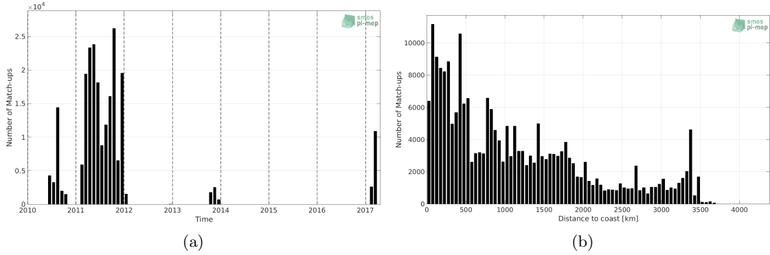
Figure 1: Number of match-ups between TSG-GOSUD-Sailing-ship and SMOS-L3-CATDS-CPDC-V317-10DAYS-25KM SSS as a function of time (a) and as function of the distance to coast (b) over the Pacific Ocean Pi-MEP region and for the full satellite product period.
