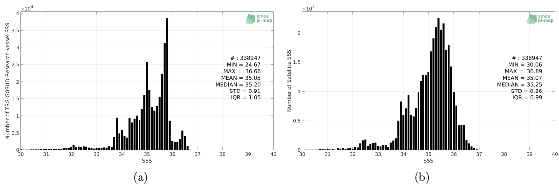
Figure 2: Histograms of SSS from TSG-GOSUD-Research-vessel (a) and SMOS L3 v317 - 10 Days - 25 km (CATDS-CPDC) (b) considering all match-up pairs per bins of 0.1 over the Pacific Ocean Pi-MEP region and for the full satellite product period.
