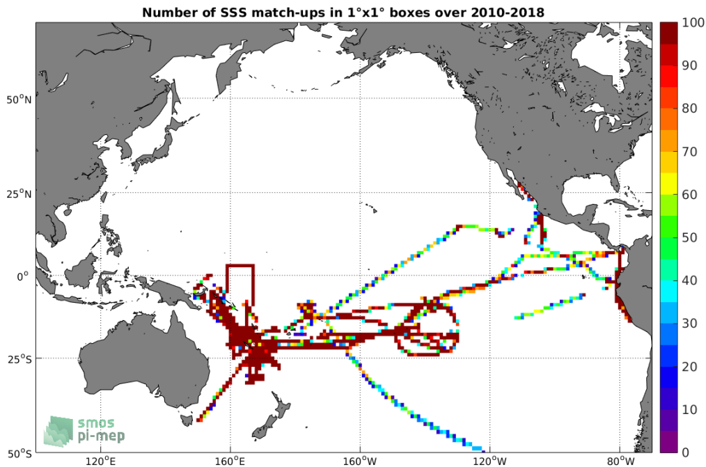
Figure 4: Number of SSS match-ups between TSG-GOSUD-Research-vessel SSS and the SMOS L3 v317 - 10 Days - 25 km (CATDS-CPDC) SSS product for the Pacific Ocean Pi-MEP region over 1^\circ \times 1^\circ boxes and for the full satellite product period.
