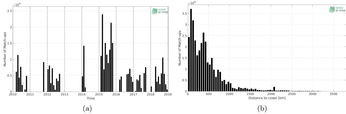
Figure 1: Number of match-ups between TSG-GOSUD-Research-vessel and SMOS L3 v317 - 10 Days - 25 km (CATDS-CPDC) SSS as a function of time (a) and as function of the distance to coast (b) over the Pacific Ocean Pi-MEP region and for the full satellite product period.
