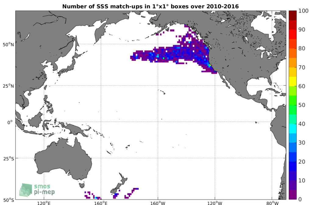
Figure 4: Number of SSS match-ups between Sea mammals SSS and the SMOS L3 v317 - 10 Days - 25 km (CATDS-CPDC) SSS product for the Pacific Ocean Pi-MEP region over 1°x1° boxes and for the full satellite product period.
