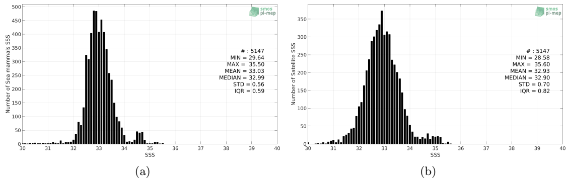
Figure 2: Histograms of SSS from Sea mammals (a) and SMOS L3 v317 - 10 Days - 25 km (CATDS-CPDC) (b) considering all match-up pairs per bins of 0.1 over the Pacific Ocean Pi-MEP region and for the full satellite product period.
