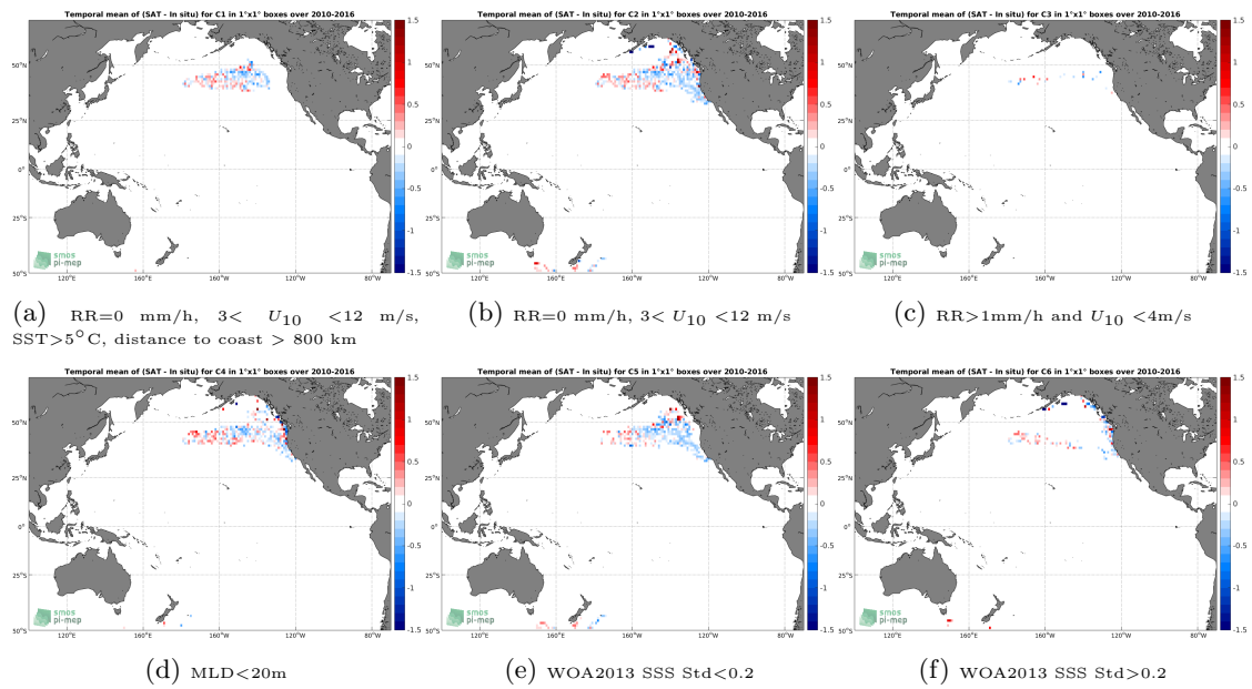
Figure 12: Temporal mean gridded over spatial boxes of size 1^\circ \times 1^\circ of \Delta SSS (SMOS L3 v317 - 10 Days - 25 km (CATDS-CPDC) - Sea mammals) for 6 different subdatasets corresponding to:RR=0 mm/h, 3 < U_{10} < 12 m/s, SST > 5^\circ C, distance to coast > 800 km (a), RR=0 mm/h, 3 < U_{10} < 12 m/s (b), RR > 1 mm/h and U_{10} < 4 m/s (c),MLD < 20 m (d),WOA2013 SSS Std < 0.2 (e),WOA2013 SSS Std > 0.2 (f).
