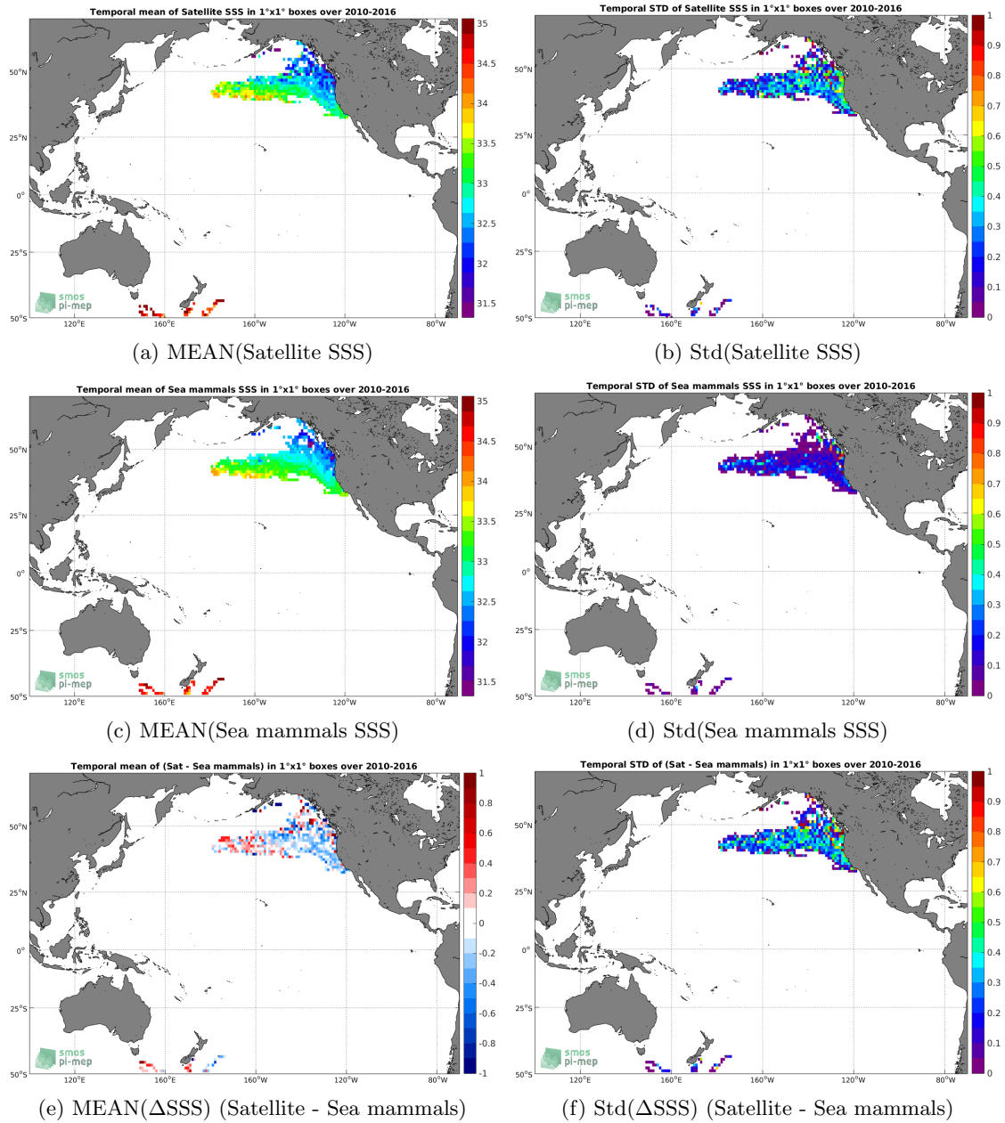
Figure 6: Temporal mean (left) and Std (right) of SSS from SMOS L3 v317 - 10 Days - 25 km (CATDS-CPDC) (top), Sea mammals (middle), and of \Delta SSS (Satellite - Sea mammals). Only match-up pairs are used to generate these maps.
