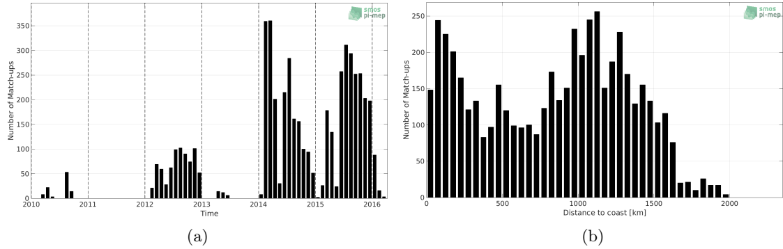
Figure 1: Number of match-ups between Sea mammals and SMOS L3 v317 - 10 Days - 25 km (CATDS-CPDC) SSS as a function of time (a) and as function of the distance to coast (b) over the Pacific Ocean Pi-MEP region and for the full satellite product period.
