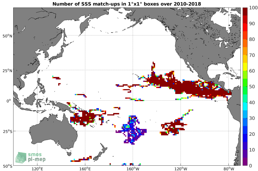
Figure 3: Number of SSS match-ups between Surface drifters SSS and the SMOS SSS L3 v317 - 10 Days - 25 km (CATDS-CPDC) SSS product for the Pacific Ocean Pi-MEP region over 1^\circ \times 1^\circ boxes and for the full satellite product period.
