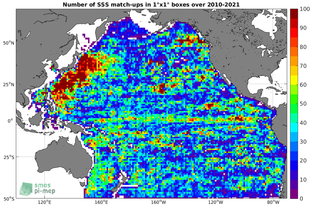
Figure 4: Number of SSS match-ups between Argo SSS and the SMOS SSS L3 v317 - 10 Days - 25 km (CATDS-CPDC) SSS product for the Pacific Ocean Pi-MEP region over 1^\circ \times 1^\circ boxes and for the full satellite product period.
