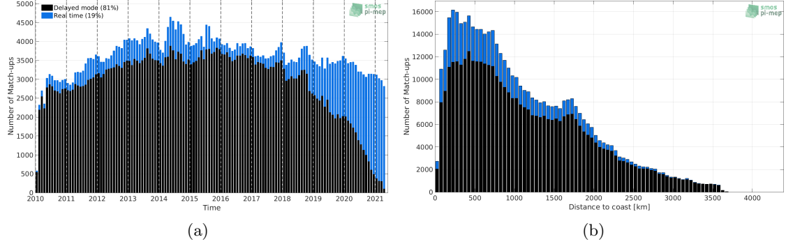
Figure 1: Number of match-ups between Argo and SMOS SSS L3 v317 - 10 Days - 25 km (CATDS-CPDC) SSS as a function of time (a) and as function of the distance to coast (b) over the Pacific Ocean Pi-MEP region and for the full satellite product period.
