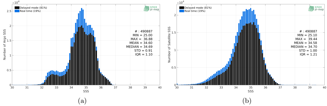
Figure 2: Histograms of SSS from Argo (a) and SMOS SSS L3 v317 - 10 Days - 25 km (CATDS-CPDC) (b) considering all match-up pairs per bins of 0.1 over the Pacific Ocean Pi-MEP region and for the full satellite product period.
