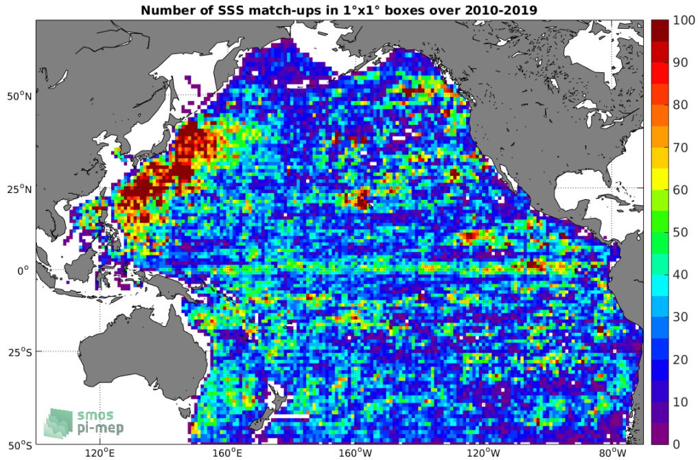
Figure 4: Number of SSS match-ups between Argo SSS and the SMOS-L3-CATDS-CPDC-V317-10DAYS-25KM SSS product for the Pacific Ocean Pi-MEP region over 1^\circ \times 1^\circ boxes and for the full satellite product period.
