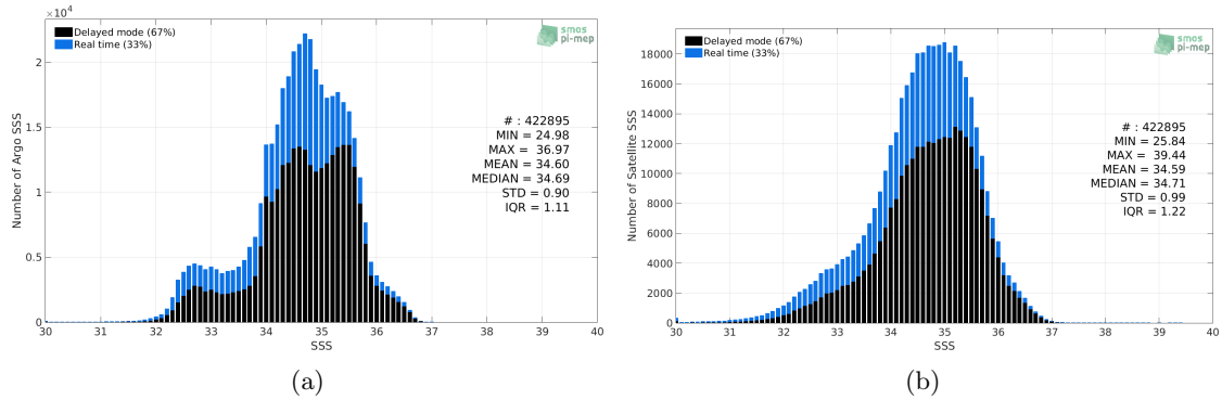
Figure 2: Histograms of SSS from Argo (a) and SMOS-L3-CATDS-CPDC-V317-10DAYS-25KM (b) considering all match-up pairs per bins of 0.1 over the Pacific Ocean Pi-MEP region and for the full satellite product period.
