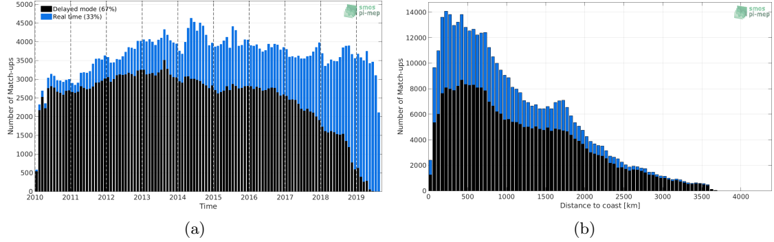
Figure 1: Number of match-ups between Argo and SMOS-L3-CATDS-CPDC-V317-10DAYS-25KM SSS as a function of time (a) and as function of the distance to coast (b) over the Pacific Ocean Pi-MEP region and for the full satellite product period.
