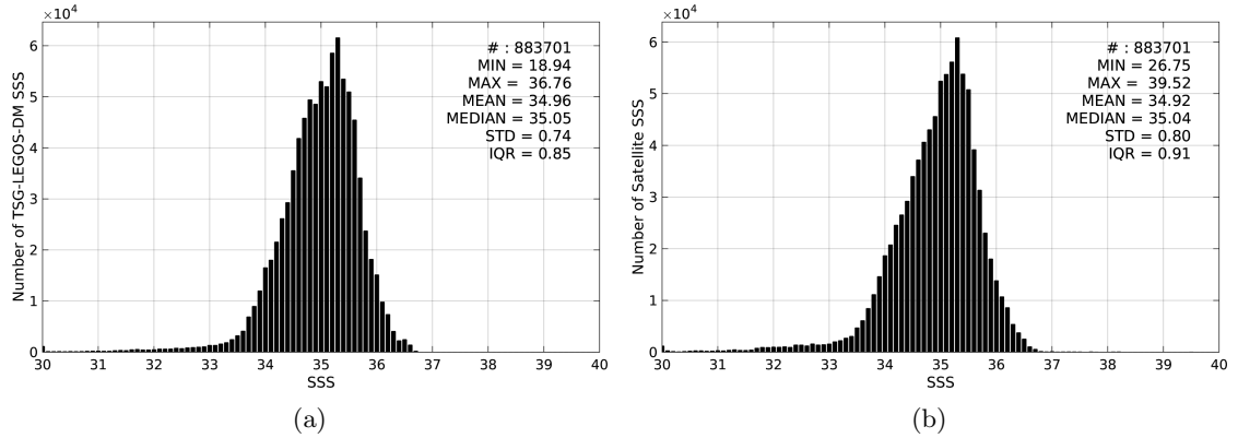
Figure 2: Histograms of SSS from TSG-LEGOS-DM (a) and SMOS-L3-CATDS-CPDC-V3-MONTHLY-25KM (b) considering all match-up pairs per bins of 0.1 over the Pacific Ocean Pi-MEP region and for the full satellite product period.
