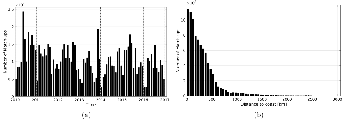
Figure 1: Number of match-ups between TSG-LEGOS-DM and SMOS-L3-CATDS-CPDC-V3-MONTHLY-25KM SSS as a function of time (a) and as function of the distance to coast (b) over the Pacific Ocean Pi-MEP region and for the full satellite product period.
