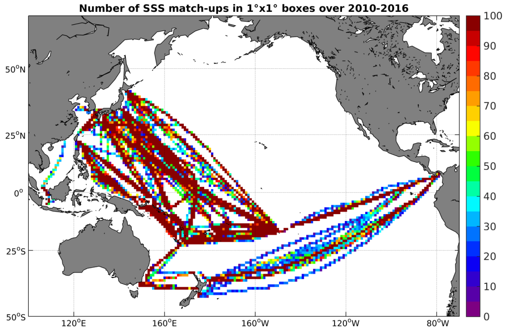
Figure 4: Number of SSS match-ups between TSG-LEGOS-DM SSS and the SMOS-L3-CATDS-CPDC-V3-MONTHLY-25KM SSS product for the Pacific Ocean Pi-MEP region over 1^\circ \times 1^\circ boxes and for the full satellite product period.
