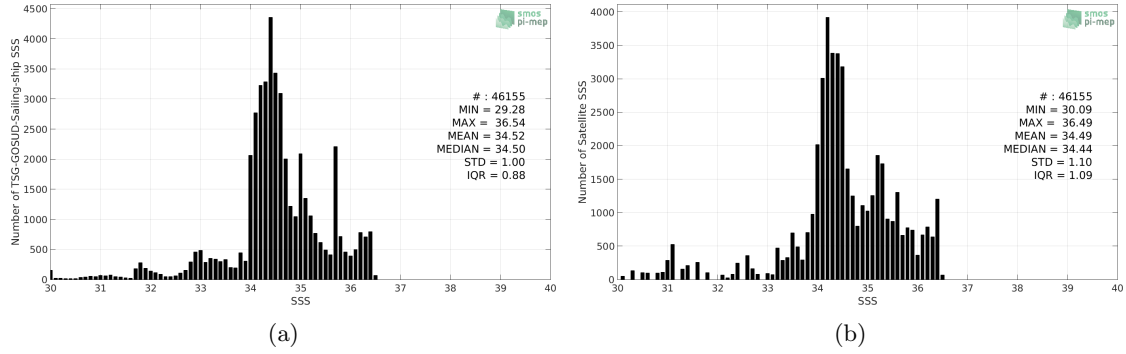
Figure 2: Histograms of SSS from TSG-GOSUD-Sailing-ship (a) and SMOS-L3-CATDS-CPDC-V3-MONTHLY-25KM (b) considering all match-up pairs per bins of 0.1 over the Pacific Ocean Pi-MEP region and for the full satellite product period.
