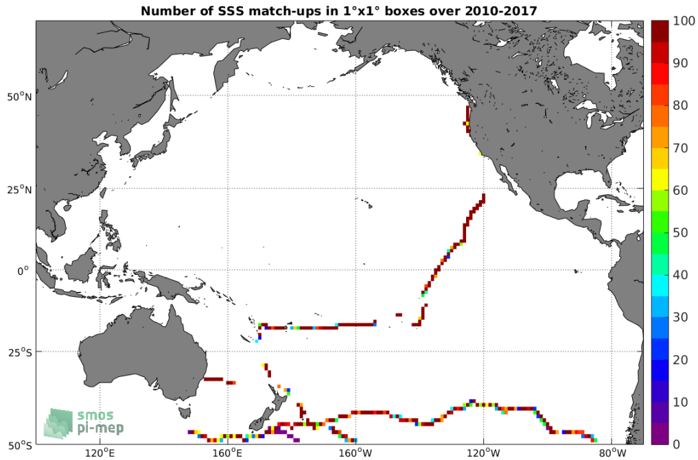
Figure 4: Number of SSS match-ups between TSG-GOSUD-Sailing-ship SSS and the SMOS-L3-CATDS-CPDC-V3-MONTHLY-25KM SSS product for the Pacific Ocean Pi-MEP region over 1^\circ \times 1^\circ boxes and for the full satellite product period.
