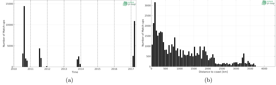
Figure 1: Number of match-ups between TSG-GOSUD-Sailing-ship and SMOS-L3-CATDS-CPDC-V3-MONTHLY-25KM SSS as a function of time (a) and as function of the distance to coast (b) over the Pacific Ocean Pi-MEP region and for the full satellite product period.
