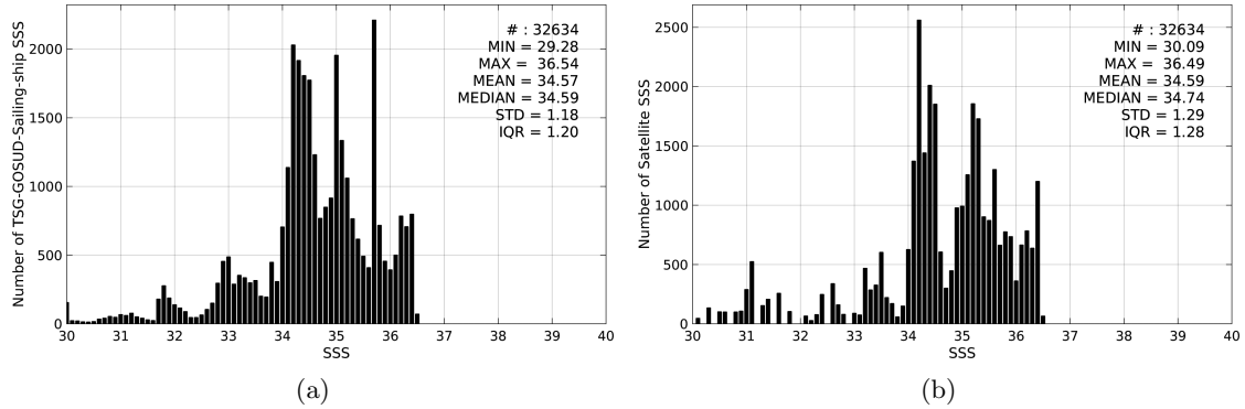
Figure 2: Histograms of SSS from TSG-GOSUD-Sailing-ship (a) and SMOS-L3-CATDS-CPDC-V3-MONTHLY-25KM (b) considering all match-up pairs per bins of 0.1 over the Pacific Ocean Pi-MEP region and for the full satellite product period.
