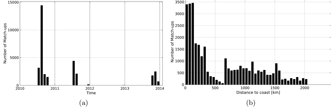
Figure 1: Number of match-ups between TSG-GOSUD-Sailing-ship and SMOS-L3-CATDS-CPDC-V3-MONTHLY-25KM SSS as a function of time (a) and as function of the distance to coast (b) over the Pacific Ocean Pi-MEP region and for the full satellite product period.
