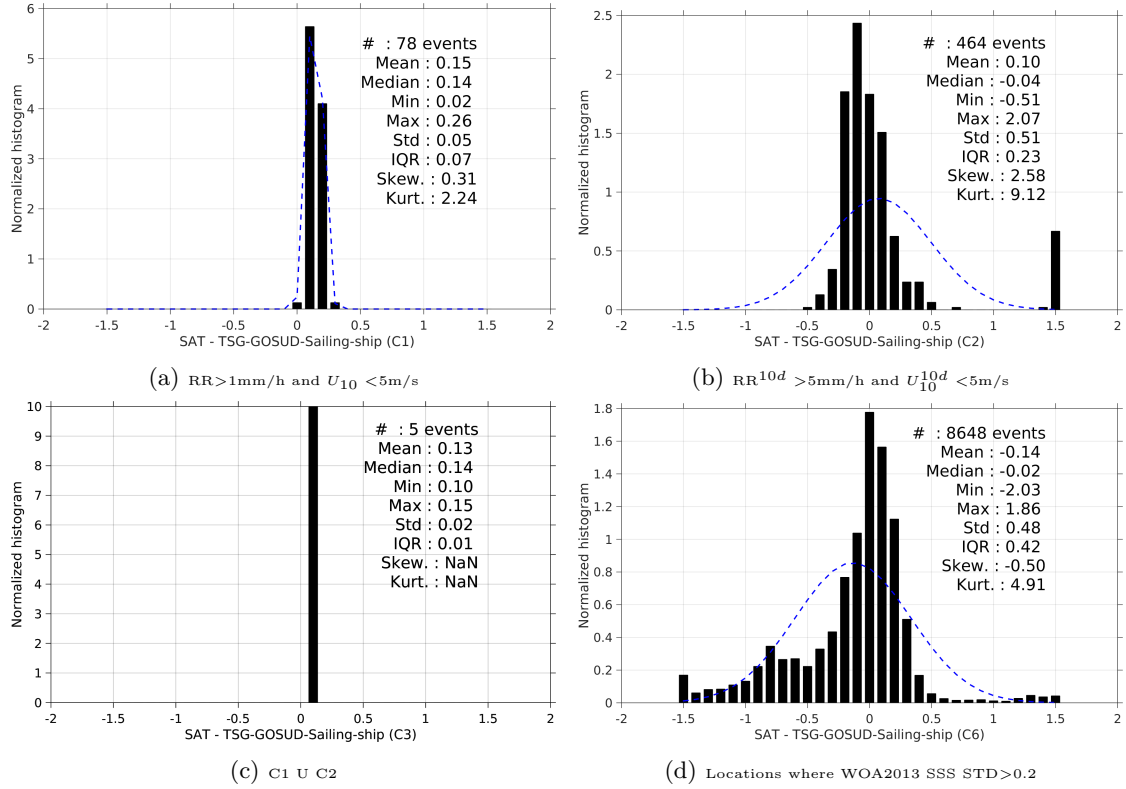
Figure 13: Normalized histogram of \Delta SSS (SMOS-L3-CATDS-CPDC-V3-MONTHLY-25KM - TSG-GOSUD-Sailing-ship) for 6 different subdatasets corresponding to: RR>1mm/h and U_{10} < 5\text{m/s} (a), RR^{10d} > 5\text{mm/h} and U_{10}^{10d} < 5\text{m/s} (b), C1 U C2 (c), Locations where WOA2013 SSS STD>0.2 (d).
