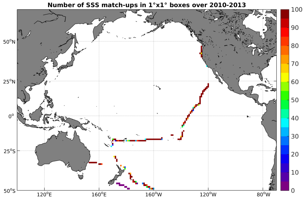
Figure 4: Number of SSS match-ups between TSG-GOSUD-Sailing-ship SSS and the SMOS-L3-CATDS-CPDC-V3-MONTHLY-25KM SSS product for the Pacific Ocean Pi-MEP region over 1^\circ \times 1^\circ boxes and for the full satellite product period.
