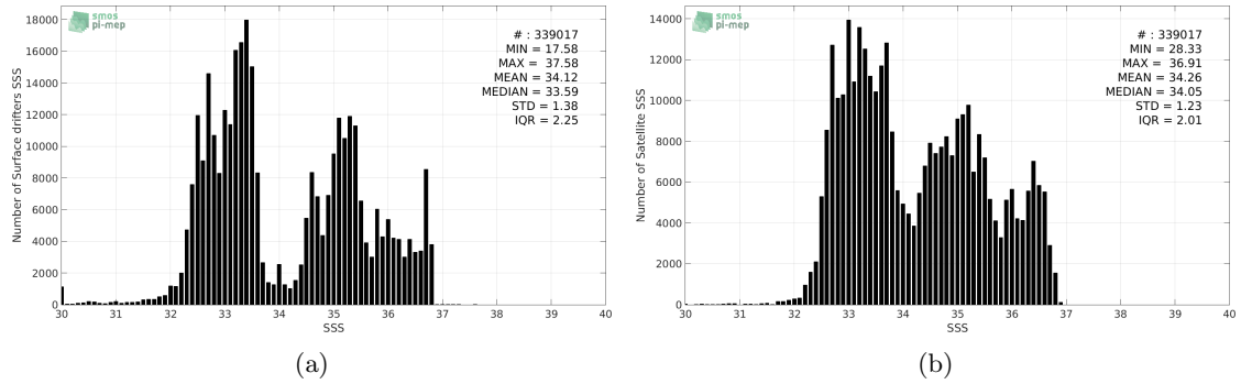
Figure 2: Histograms of SSS from Surface drifters (a) and SMOS-L3-CATDS-CPDC-V3-MONTHLY-25KM (b) considering all match-up pairs per bins of 0.1 over the Pacific Ocean Pi-MEP region and for the full satellite product period.
