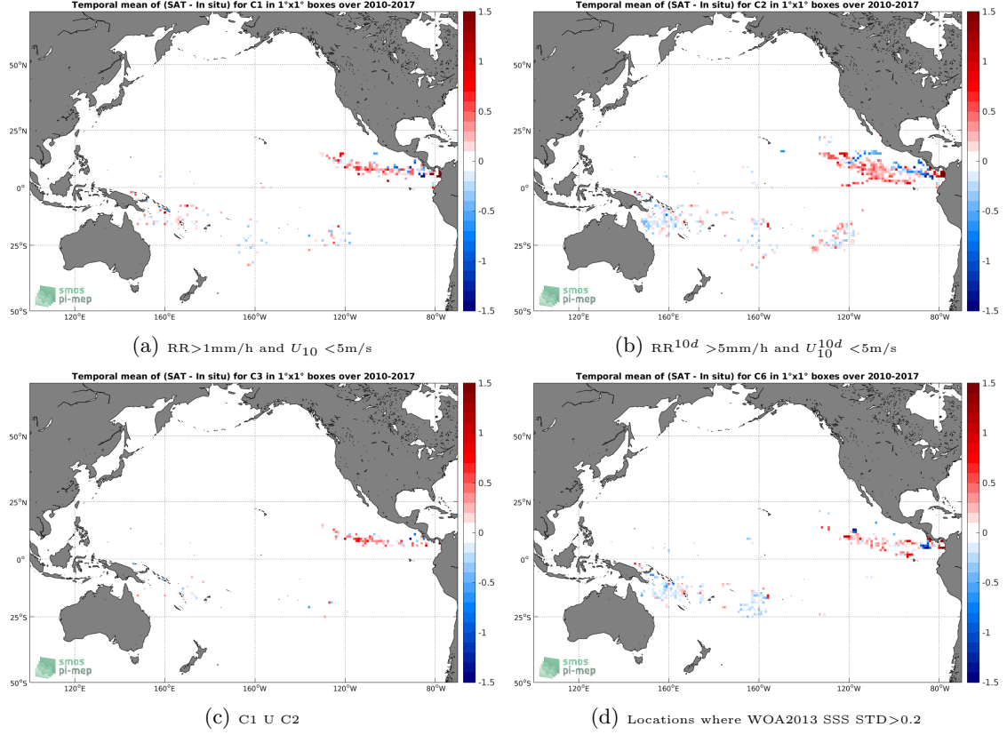
Figure 11: Temporal mean gridded over spatial boxes of size 1^\circ \times 1^\circ of \Delta SSS (SMOS-L3-CATDS-CPDC-V3-MONTHLY-25KM - Surface drifters) for 4 different subdatasets corresponding to: RR > 1\text{mm/h} and U_{10} < 5\text{m/s} (a), RR^{10d} > 5\text{mm/h} and U_{10}^{10d} < 5\text{m/s} (b), C1 U C2 (c), Locations where WOA2013 SSS STD > 0.2 (d).
