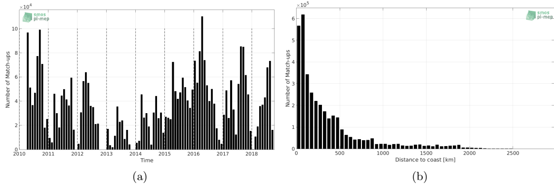
Figure 1: Number of match-ups between TSG-SAMOS and SMOS-L3-CATDS-CPDC-V3-10DAYS-25KM SSS as a function of time (a) and as function of the distance to coast (b) over the Pacific Ocean Pi-MEP region and for the full satellite product period.
