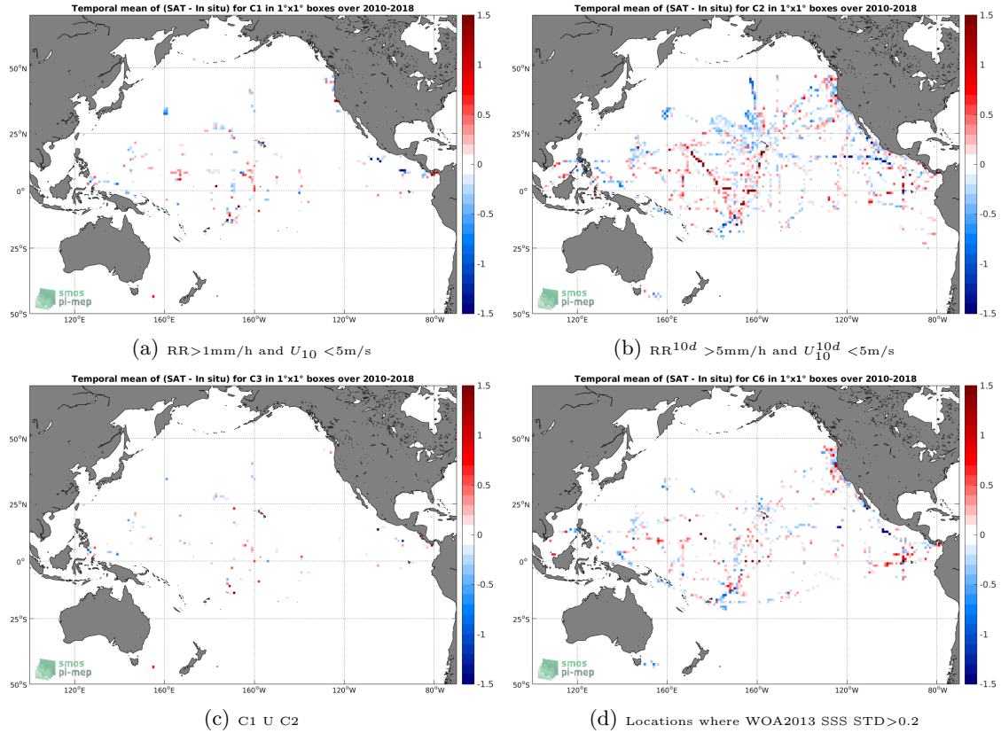
Figure 12: Temporal mean gridded over spatial boxes of size 1^\circ \times 1^\circ of \Delta SSS (SMOS-L3-CATDS-CPDC-V3-10DAYS-25KM - TSG-SAMOS) for 4 different subdatasets corresponding to: RR > 1mm/h and U_{10} < 5\text{m/s} (a), RR^{10d} > 5\text{mm/h} and U_{10}^{10d} < 5\text{m/s} (b), C1 U C2 (c), Locations where WOA2013 SSS STD > 0.2 (d).
