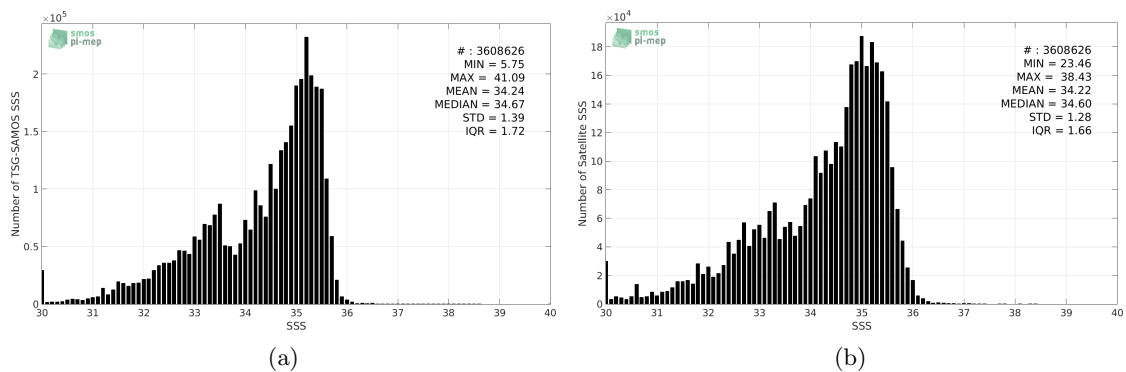
Figure 2: Histograms of SSS from TSG-SAMOS (a) and SMOS-L3-CATDS-CPDC-V3-10DAYS-25KM (b) considering all match-up pairs per bins of 0.1 over the Pacific Ocean Pi-MEP region and for the full satellite product period.
