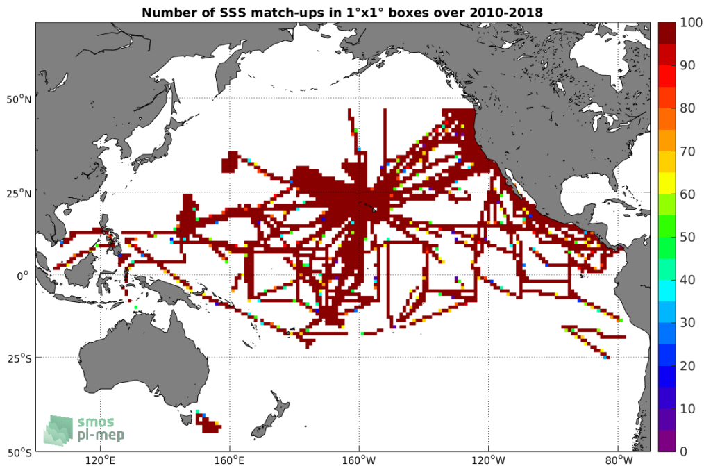
Figure 4: Number of SSS match-ups between TSG-SAMOS SSS and the SMOS-L3-CATDS-CPDC-V3-10DAYS-25KM SSS product for the Pacific Ocean Pi-MEP region over 1^\circ \times 1^\circ boxes and for the full satellite product period.
