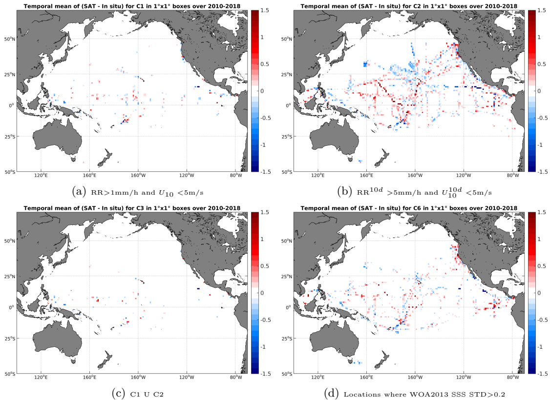
Figure 12: Temporal mean gridded over spatial boxes of size 1^\circ \times 1^\circ of \Delta SSS (SMOS-L3-CATDS-CPDC-V3-10DAYS-25KM - TSG-SAMOS) for 4 different subdatasets corresponding to: RR > 1\text{mm/h} and U_{10} < 5\text{m/s} (a), RR^{10d} > 5\text{mm/h} and U_{10}^{10d} < 5\text{m/s} (b), C1 U C2 (c), Locations where WOA2013 SSS STD > 0.2 (d).
