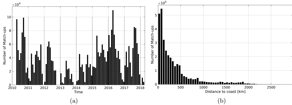
Figure 1: Number of match-ups between TSG-SAMOS and SMOS-L3-CATDS-CPDC-V3-10DAYS-25KM SSS as a function of time (a) and as function of the distance to coast (b) over the Pacific Ocean Pi-MEP region and for the full satellite product period.
