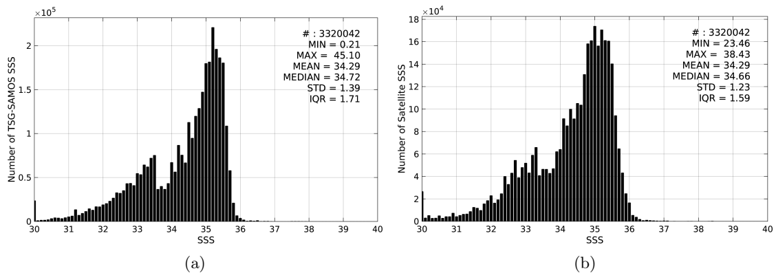
Figure 2: Histograms of SSS from TSG-SAMOS (a) and SMOS-L3-CATDS-CPDC-V3-10DAYS-25KM (b) considering all match-up pairs per bins of 0.1 over the Pacific Ocean Pi-MEP region and for the full satellite product period.
