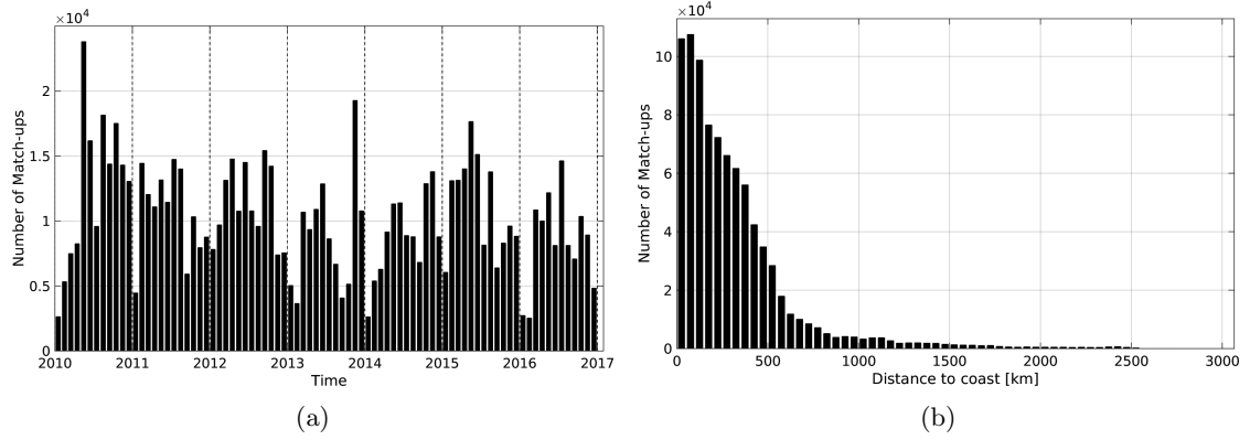
Figure 1: Number of match-ups between TSG-LEGOS-DM and SMOS-L3-CATDS-CPDC-V3-10DAYS-25KM SSS as a function of time (a) and as function of the distance to coast (b) over the Pacific Ocean Pi-MEP region and for the full satellite product period.
