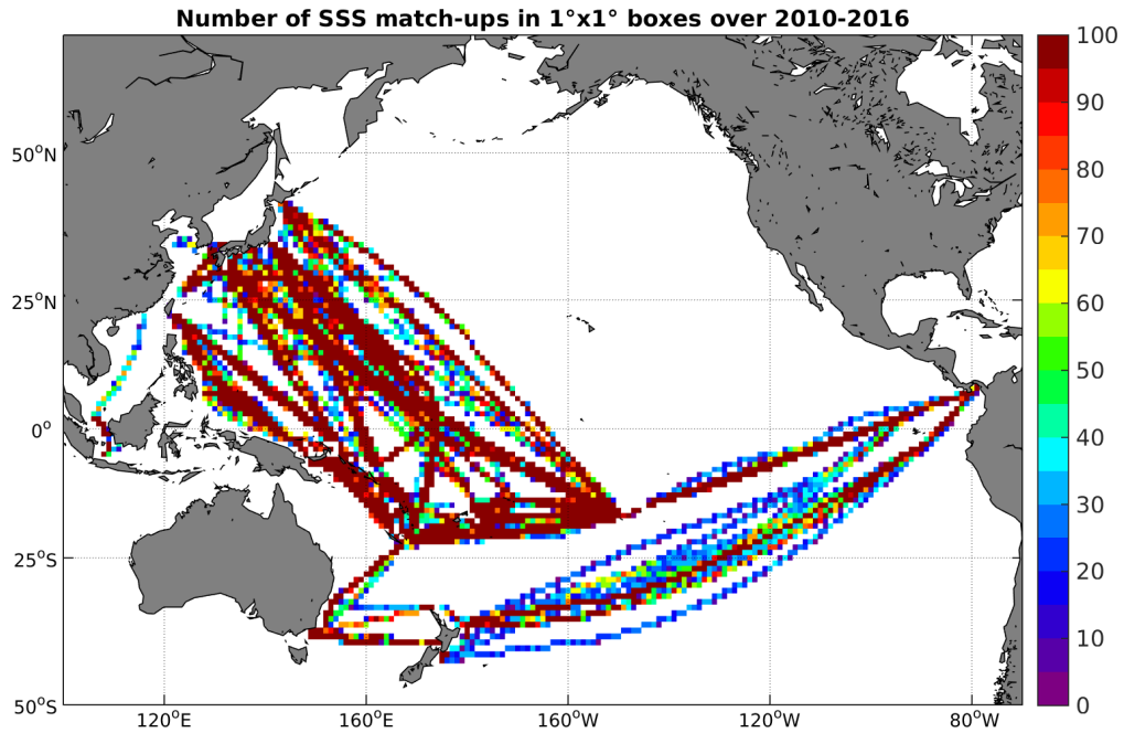
Figure 4: Number of SSS match-ups between TSG-LEGOS-DM SSS and the SMOS-L3-CATDS-CPDC-V3-10DAYS-25KM SSS product for the Pacific Ocean Pi-MEP region over 1^\circ \times 1^\circ boxes and for the full satellite product period.
