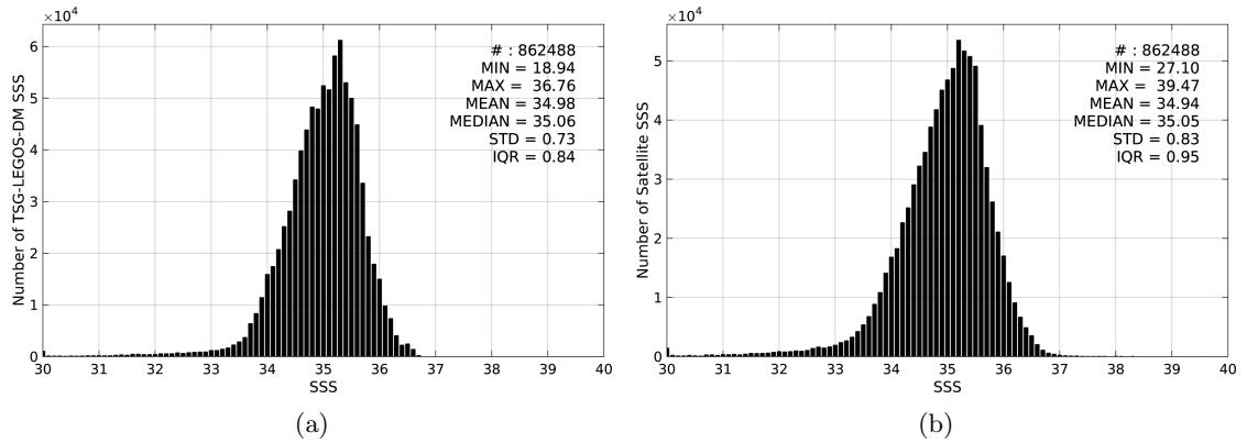
Figure 2: Histograms of SSS from TSG-LEGOS-DM (a) and SMOS-L3-CATDS-CPDC-V3-10DAYS-25KM (b) considering all match-up pairs per bins of 0.1 over the Pacific Ocean Pi-MEP region and for the full satellite product period.
