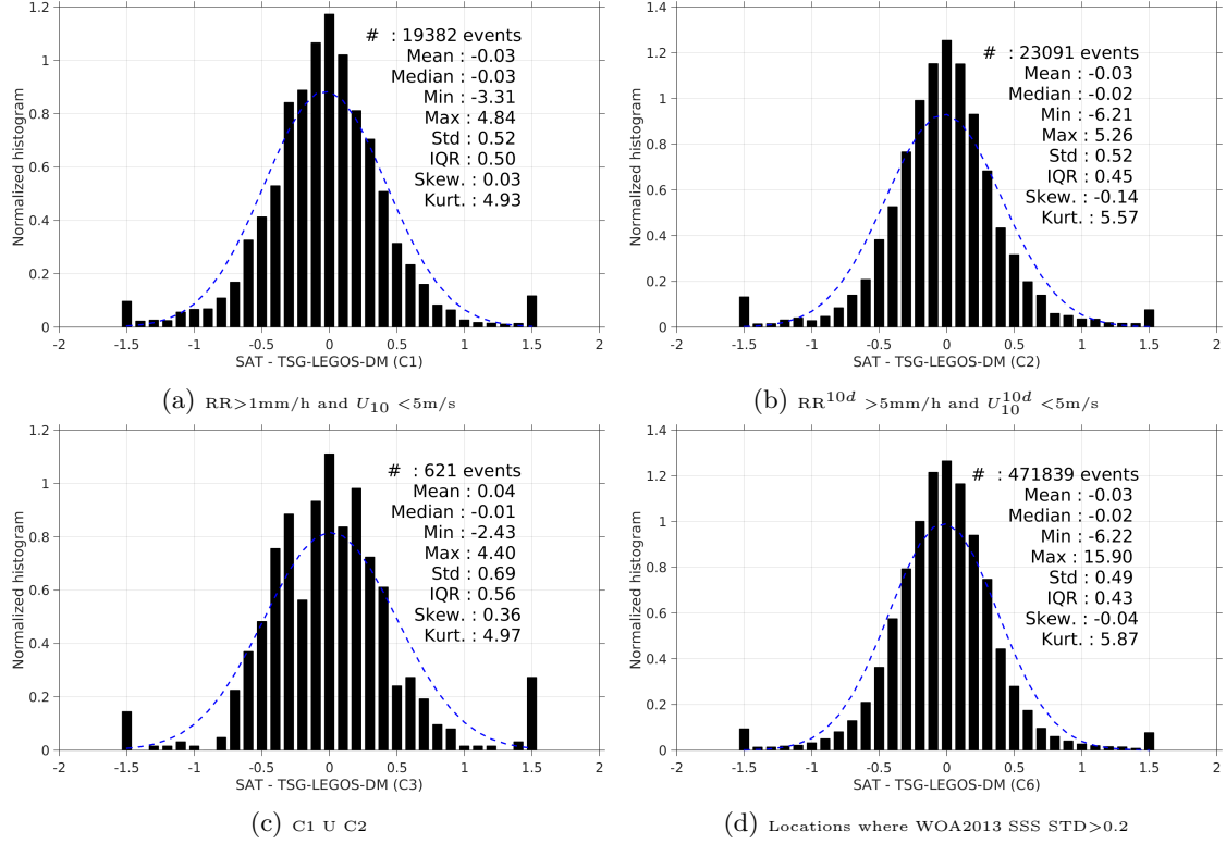
Figure 13: Normalized histogram of \Delta SSS (SMOS-L3-CATDS-CPDC-V3-10DAYS-25KM - TSG-LEGOS-DM) for 6 different subdatasets corresponding to: RR > 1\text{mm/h} and U_{10} < 5\text{m/s} (a), RR^{10d} > 5\text{mm/h} and U_{10}^{10d} < 5\text{m/s} (b), C1 U C2 (c), Locations where WOA2013 SSS STD > 0.2 (d).
