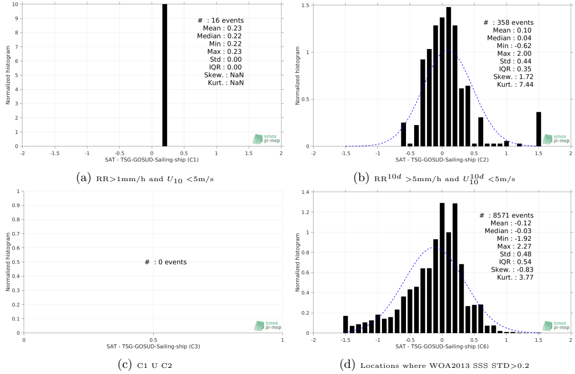
Figure 13: Normalized histogram of \Delta\text{SSS} (SMOS-L3-CATDS-CPDC-V3-10DAYS-25KM - TSG-GOSUD-Sailing-ship) for 6 different subdatasets corresponding to: RR > 1mm/h and U_{10} < 5\text{m/s} (a), RR^{10d} > 5\text{mm/h} and U_{10}^{10d} < 5\text{m/s} (b), C1 U C2 (c), Locations where WOA2013 SSS STD > 0.2 (d).
