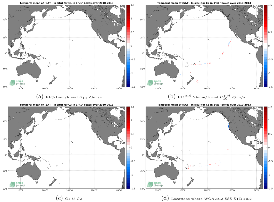
Figure 12: Temporal mean gridded over spatial boxes of size 1^\circ \times 1^\circ of \Delta SSS (SMOS-L3-CATDS-CPDC-V3-10DAYS-25KM - TSG-GOSUD-Sailing-ship) for 4 different subdatasets corresponding to: RR > 1mm/h and U_{10} < 5\text{m/s} (a), RR^{10d} > 5\text{mm/h} and U_{10}^{10d} < 5\text{m/s} (b), C1 U C2 (c), Locations where WOA2013 SSS STD > 0.2 (d).
