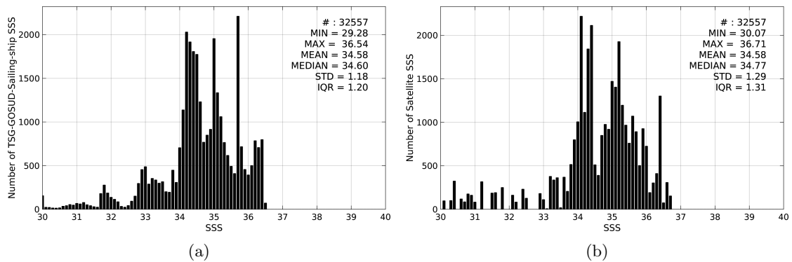
Figure 2: Histograms of SSS from TSG-GOSUD-Sailing-ship (a) and SMOS-L3-CATDS-CPDC-V3-10DAYS-25KM (b) considering all match-up pairs per bins of 0.1 over the Pacific Ocean Pi-MEP region and for the full satellite product period.
