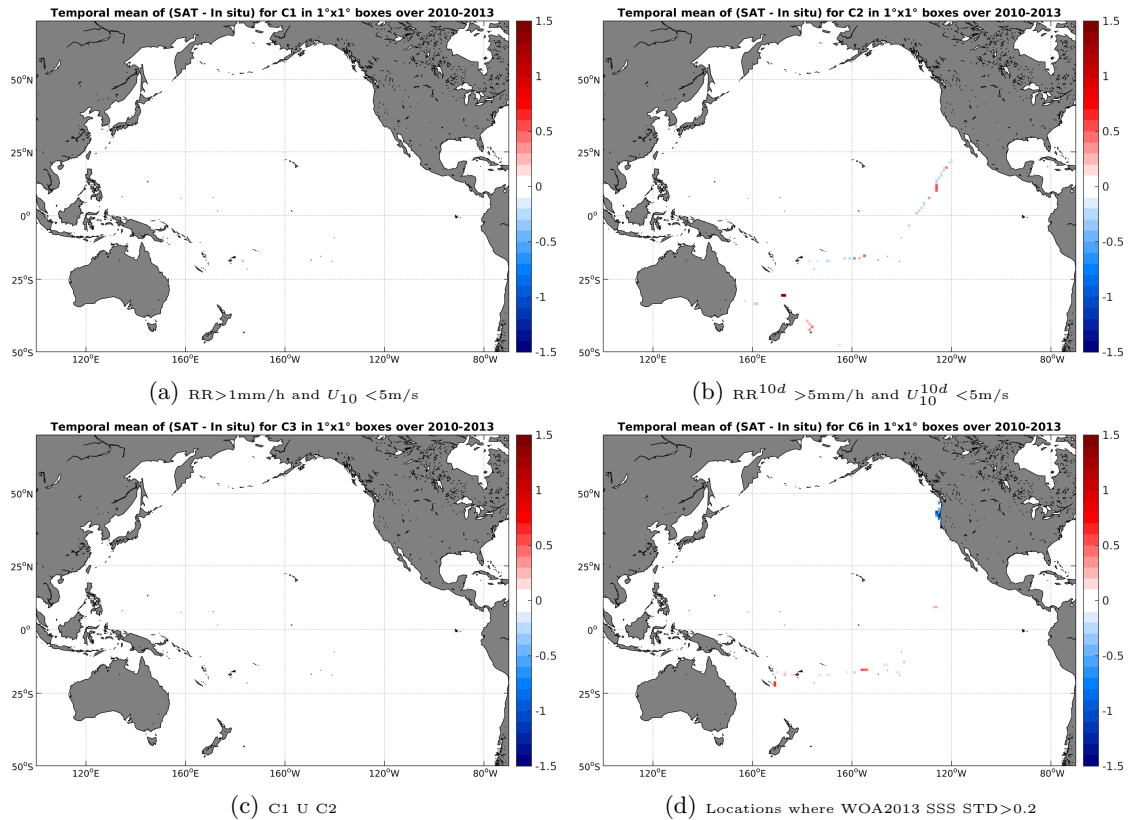
Figure 12: Temporal mean gridded over spatial boxes of size 1°x1° of \Delta SSS (SMOS-L3-CATDS-CPDC-V3-10DAYS-25KM - TSG-GOSUD-Sailing-ship) for 4 different subdatasets corresponding to: RR > 1\text{mm/h} and U_{10} < 5\text{m/s} (a), RR^{10d} > 5\text{mm/h} and U_{10}^{10d} < 5\text{m/s} (b), C1 U C2 (c), Locations where WOA2013 SSS STD > 0.2 (d).
