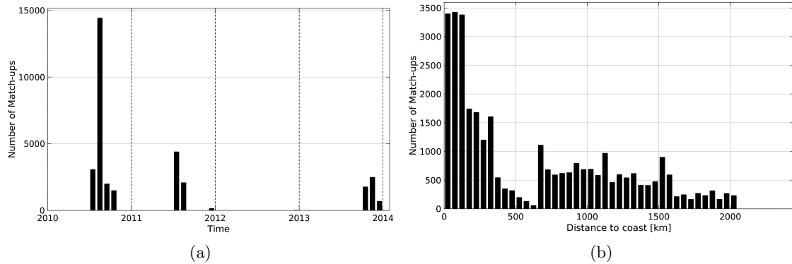
Figure 1: Number of match-ups between TSG-GOSUD-Sailing-ship and SMOS-L3-CATDS-CPDC-V3-10DAYS-25KM SSS as a function of time (a) and as function of the distance to coast (b) over the Pacific Ocean Pi-MEP region and for the full satellite product period.
