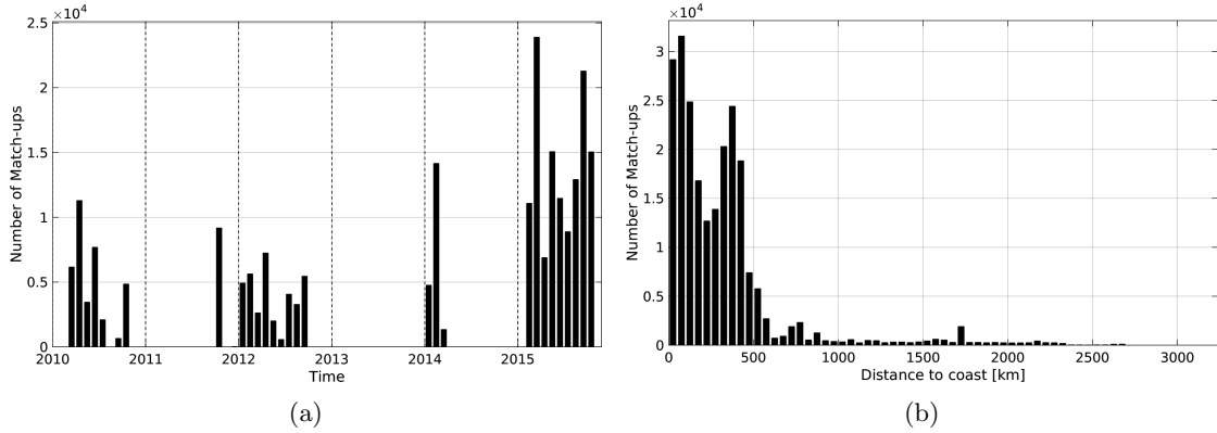
Figure 1: Number of match-ups between TSG-GOSUD-Research-vessel and SMOS-L3-CATDS-CPDC-V3-10DAYS-25KM SSS as a function of time (a) and as function of the distance to coast (b) over the Pacific Ocean Pi-MEP region and for the full satellite product period.
