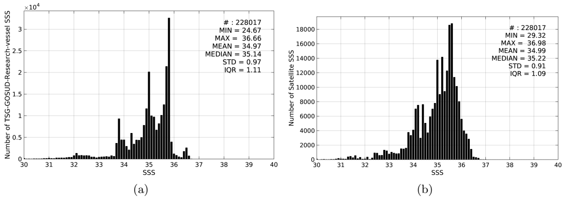
Figure 2: Histograms of SSS from TSG-GOSUD-Research-vessel (a) and SMOS-L3-CATDS-CPDC-V3-10DAYS-25KM (b) considering all match-up pairs per bins of 0.1 over the Pacific Ocean Pi-MEP region and for the full satellite product period.
