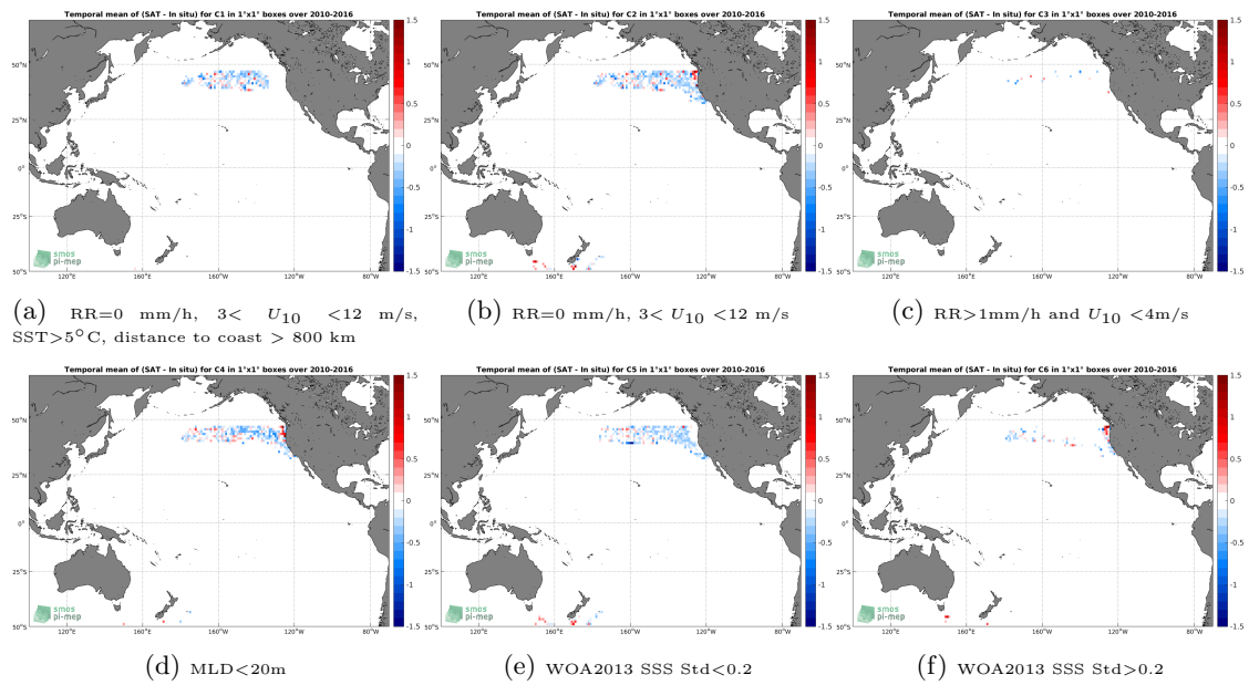
Figure 12: Temporal mean gridded over spatial boxes of size 1^\circ \times 1^\circ of \Delta SSS (SMOS-L3-CATDS-CPDC-V3-10DAYS-25KM - Sea mammals) for 6 different subdatasets corresponding to:RR=0 mm/h, 3 < U_{10} < 12 m/s, SST >5^\circ C, distance to coast > 800 km (a), RR=0 mm/h, 3 < U_{10} < 12 m/s (b), RR >1 mm/h and U_{10} < 4 m/s (c),MLD <20 m (d),WOA2013 SSS Std <0.2 (e),WOA2013 SSS Std >0.2 (f).
