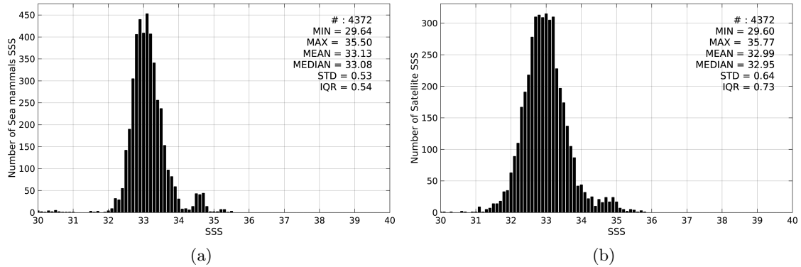
Figure 2: Histograms of SSS from Sea mammals (a) and SMOS-L3-CATDS-CPDC-V3-10DAYS-25KM (b) considering all match-up pairs per bins of 0.1 over the Pacific Ocean Pi-MEP region and for the full satellite product period.
