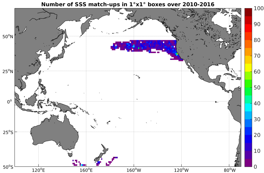
Figure 4: Number of SSS match-ups between Sea mammals SSS and the SMOS-L3-CATDS-CPDC-V3-10DAYS-25KM SSS product for the Pacific Ocean Pi-MEP region over 1^\circ \times 1^\circ boxes and for the full satellite product period.
