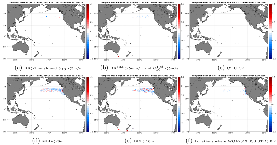
Figure 12: Temporal mean gridded over spatial boxes of size 1^\circ \times 1^\circ of \Delta SSS (SMOS-L3-CATDS-CPDC-V3-10DAYS-25KM - Sea mammals) for 6 different subdatasets corresponding to:RR>1mm/h and U_{10} < 5\text{m/s} (a), RR^{10d} > 5\text{mm/h} and U_{10}^{10d} < 5\text{m/s} (b), C1 U C2 (c),MLD<20m (d),BLT>10m (e),Locations where WOA2013 SSS STD>0.2 (f).
