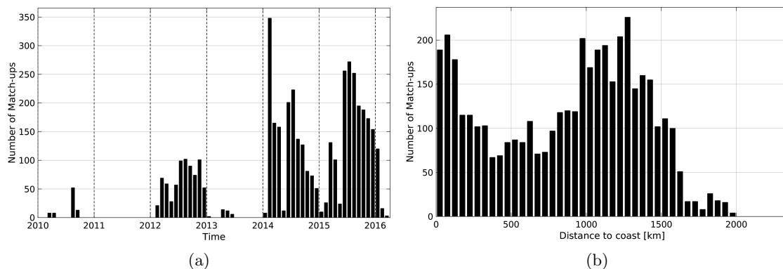
Figure 1: Number of match-ups between Sea mammals and SMOS-L3-CATDS-CPDC-V3-10DAYS-25KM SSS as a function of time (a) and as function of the distance to coast (b) over the Pacific Ocean Pi-MEP region and for the full satellite product period.
