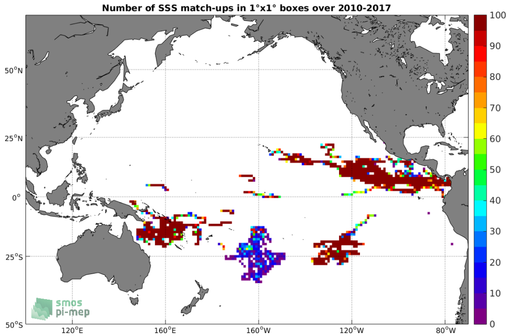
Figure 3: Number of SSS match-ups between Surface drifters SSS and the SMOS-L3-CATDS-CPDC-V3-10DAYS-25KM SSS product for the Pacific Ocean Pi-MEP region over 1^{\circ} \times 1^{\circ} boxes and for the full satellite product period.
