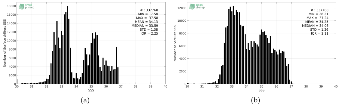
Figure 2: Histograms of SSS from Surface drifters (a) and SMOS-L3-CATDS-CPDC-V3-10DAYS-25KM (b) considering all match-up pairs per bins of 0.1 over the Pacific Ocean Pi-MEP region and for the full satellite product period.
