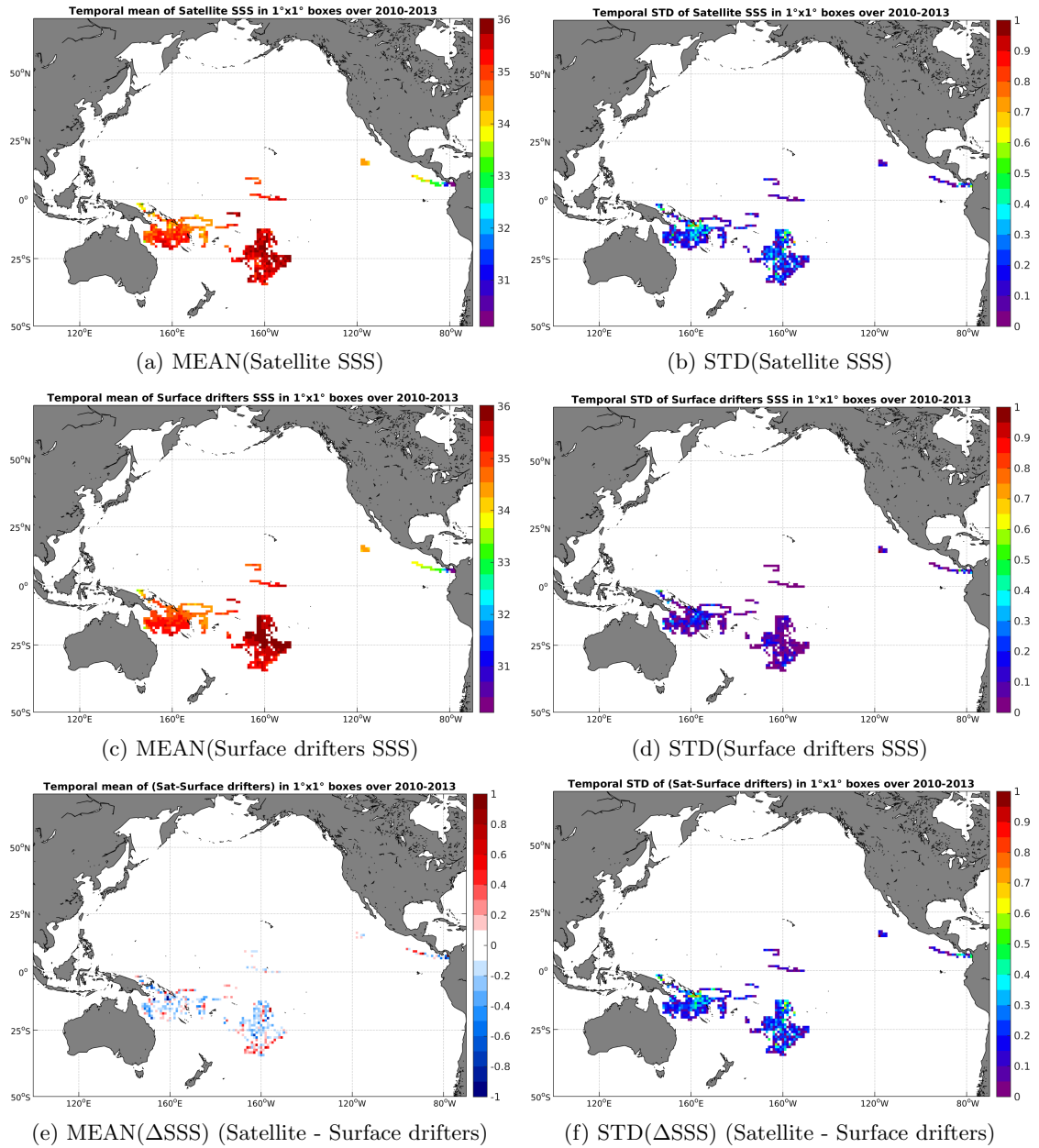
Figure 5: Temporal mean (left) and STD (right) of SSS from SMOS-L3-CATDS-CPDC-V3-10DAYS-25KM (top), Surface drifters (middle), and of \Delta SSS (Satellite - Surface drifters). Only match-up pairs are used to generate these maps.
