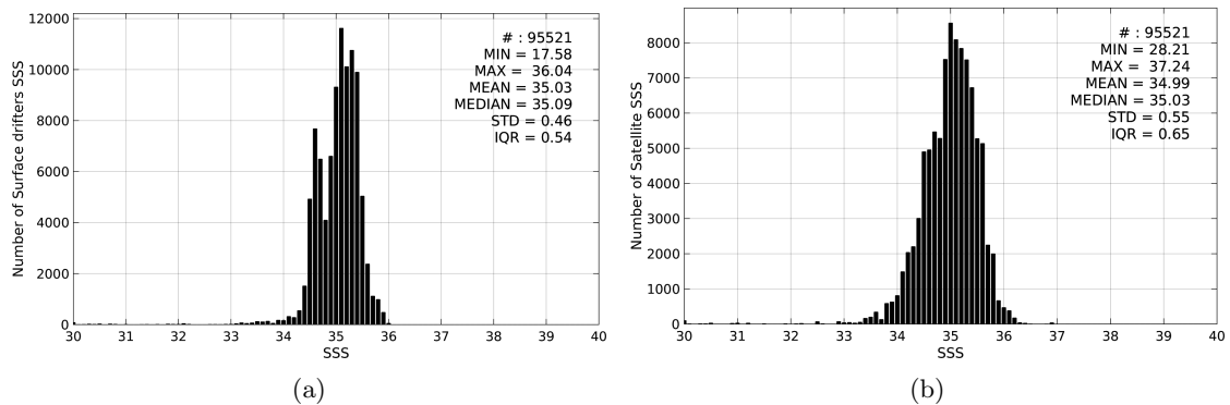
Figure 2: Histograms of SSS from Surface drifters (a) and SMOS-L3-CATDS-CPDC-V3-10DAYS-25KM (b) considering all match-up pairs per bins of 0.1 over the Pacific Ocean Pi-MEP region and for the full satellite product period.
