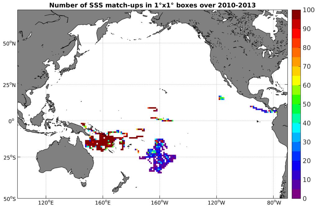
Figure 3: Number of SSS match-ups between Surface drifters SSS and the SMOS-L3-CATDS-CPDC-V3-10DAYS-25KM SSS product for the Pacific Ocean Pi-MEP region over 1^\circ \times 1^\circ boxes and for the full satellite product period.
