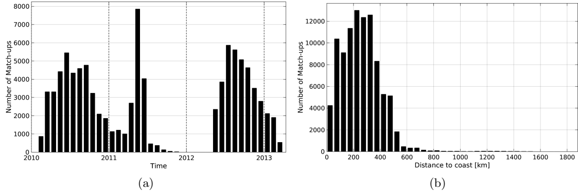
Figure 1: Number of match-ups between Surface drifters and SMOS-L3-CATDS-CPDC-V3-10DAYS-25KM SSS as a function of time (a) and as function of the distance to coast (b) over the Pacific Ocean Pi-MEP region and for the full satellite product period.
