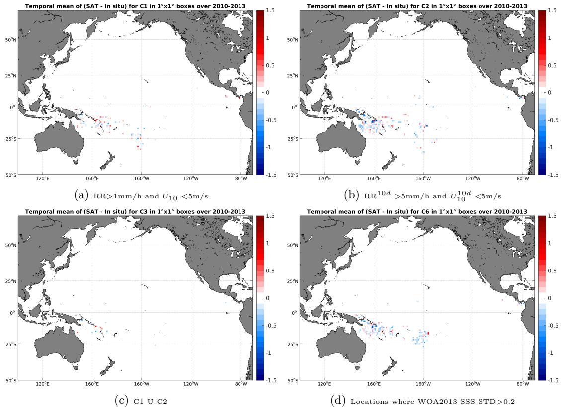
Figure 11: Temporal mean gridded over spatial boxes of size 1^\circ \times 1^\circ of \Delta SSS (SMOS-L3-CATDS-CPDC-V3-10DAYS-25KM - Surface drifters) for 4 different subdatasets corresponding to: RR > 1mm/h and U_{10} < 5 m/s (a), RR^{10d} > 5 mm/h and U_{10}^{10d} < 5 m/s (b), C1 U C2 (c), Locations where WOA2013 SSS STD > 0.2 (d).
