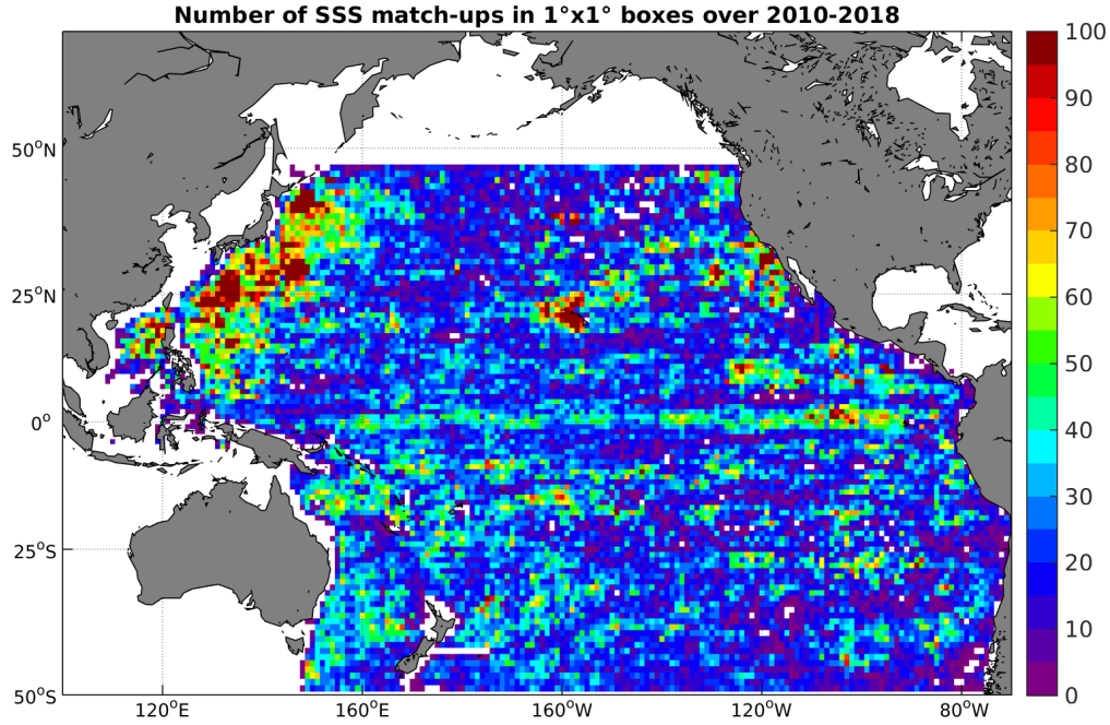
Figure 4: Number of SSS match-ups between Argo SSS and the SMOS-L3-CATDS-CPDC-V3-10DAYS-25KM SSS product for the Pacific Ocean Pi-MEP region over 1^\circ \times 1^\circ boxes and for the full satellite product period.
