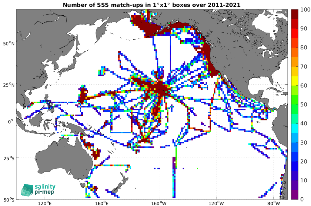
Figure 5: Number of SSS match-ups between TSG (SAMOS) SSS and the SMOS SSS L3 v2 - 9-Days (BEC) SSS product for the Pacific Ocean Pi-MEP region over 1^\circ \times 1^\circ boxes and for the full satellite product period.
