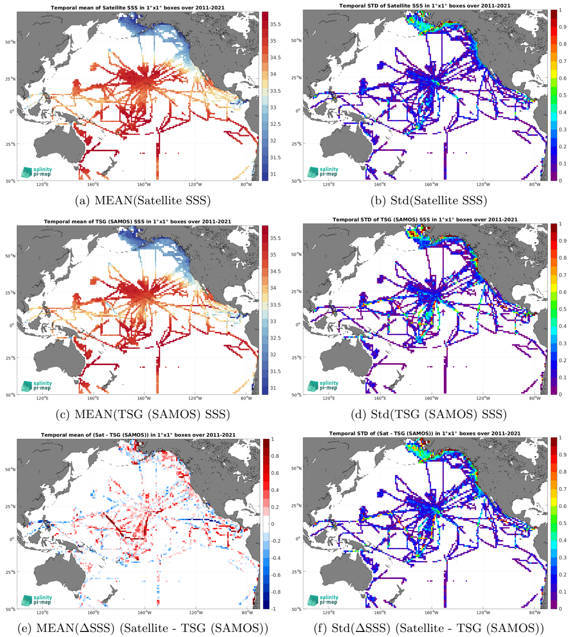
Figure 7: Temporal mean (left) and Std (right) of SSS from SMOS SSS L3 v2 - 9-Days (BEC) (top), TSG (SAMOS) (middle), and of \Delta SSS (Satellite - TSG (SAMOS)). Only match-up pairs are used to generate these maps.
