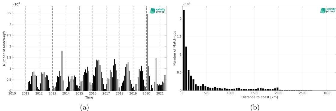
Figure 2: Number of match-ups between TSG (SAMOS) and SMOS SSS L3 v2 - 9-Days (BEC) SSS as a function of time (a) and as function of the distance to coast (b) over the Pacific Ocean Pi-MEP region and for the full satellite product period.
