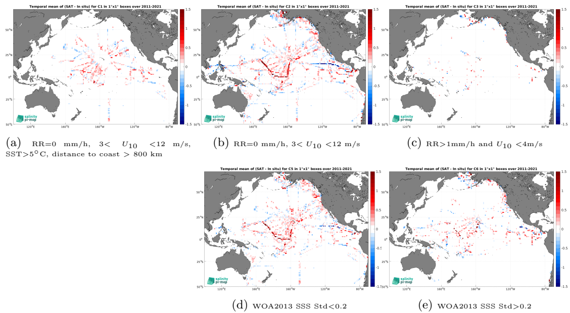
Figure 14: Temporal mean gridded over spatial boxes of size 1^\circ \times 1^\circ of \Delta SSS (SMOS SSS L3 v2 - 9-Days (BEC) - TSG (SAMOS)) for 5 different subdatasets corresponding to:RR=0 mm/h, 3 < U_{10} < 12 m/s, SST >5^\circ\text{C} , distance to coast > 800 km (a), RR=0 mm/h, 3 < U_{10} < 12 m/s (b), RR >1 mm/h and U_{10} < 4 m/s (c), WOA2013 SSS Std <0.2 (d), WOA2013 SSS Std >0.2 (e).
