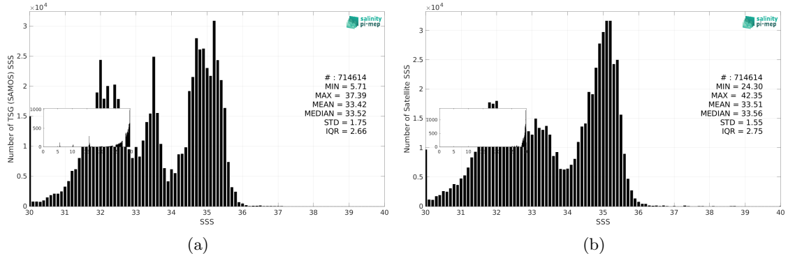
Figure 3: Histograms of SSS from TSG (SAMOS) (a) and SMOS SSS L3 v2 - 9-Days (BEC) (b) considering all match-up pairs per bins of 0.1 over the Pacific Ocean Pi-MEP region and for the full satellite product period.
