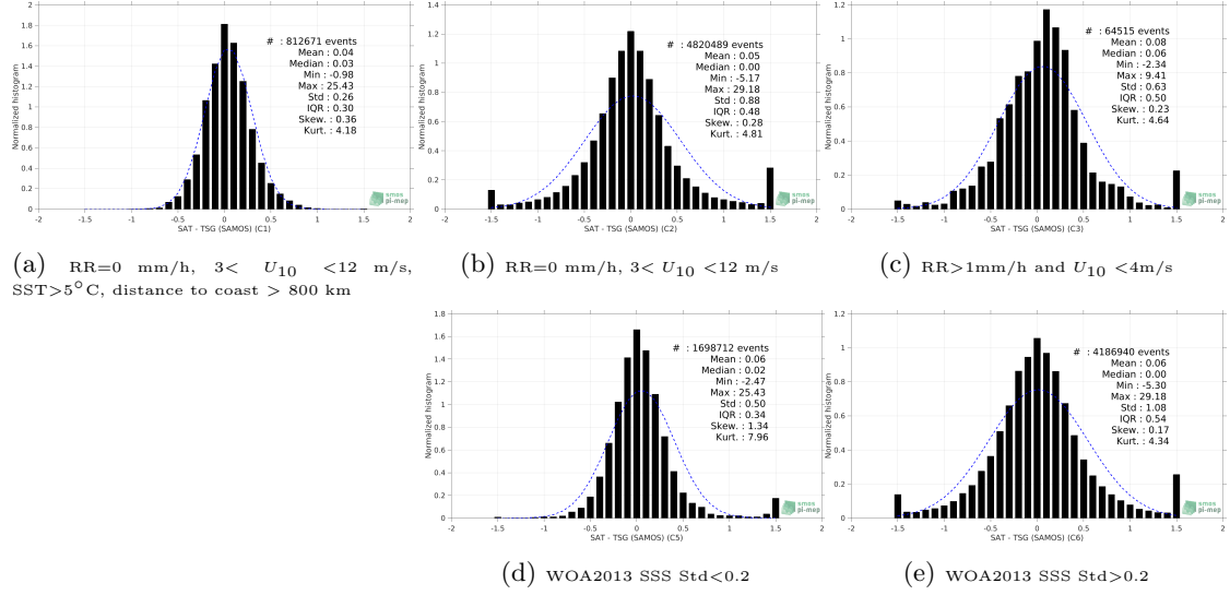
Figure 13: Normalized histogram of \Delta\text{SSS} (SMOS SSS L3 v2 - 9-Days (BEC) - TSG (SAMOS)) for 5 different subdatasets corresponding to: \text{RR}=0 \text{ mm/h} , 3 < U_{10} < 12 \text{ m/s} , \text{SST} > 5^\circ\text{C} , distance to coast > 800 \text{ km} (a), \text{RR}=0 \text{ mm/h} , 3 < U_{10} < 12 \text{ m/s} (b), \text{RR} > 1 \text{ mm/h} and U_{10} < 4 \text{ m/s} (c), WOA2013 SSS Std < 0.2 (d), WOA2013 SSS Std > 0.2 (e).
