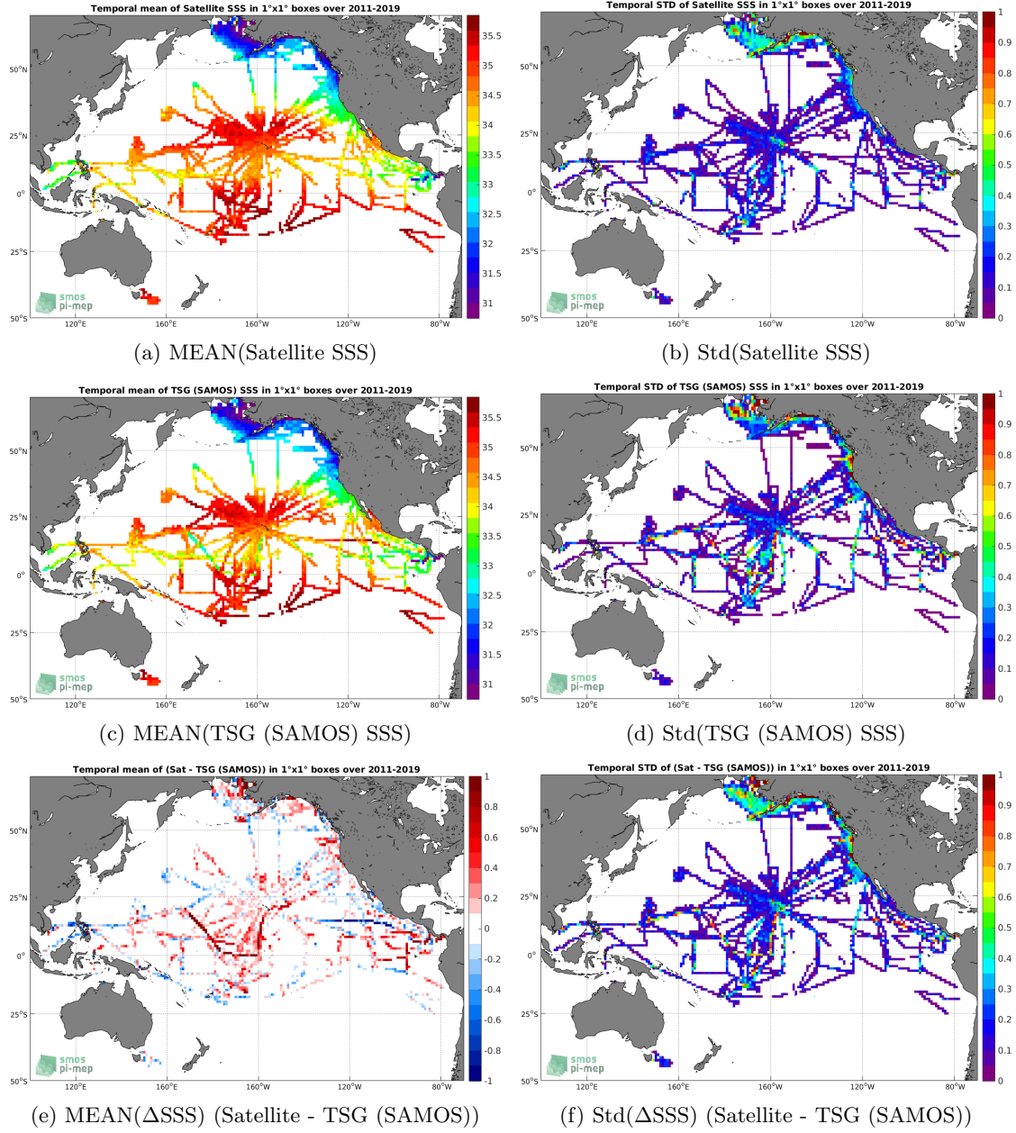
Figure 6: Temporal mean (left) and Std (right) of SSS from SMOS L3 v2 - 9-Days (BEC) (top), TSG (SAMOS) (middle), and of \Delta SSS (Satellite - TSG (SAMOS)). Only match-up pairs are used to generate these maps.
