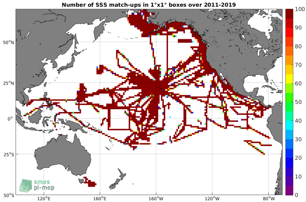
Figure 4: Number of SSS match-ups between TSG (SAMOS) SSS and the SMOS L3 v2 - 9-Days (BEC) SSS product for the Pacific Ocean Pi-MEP region over 1°x1° boxes and for the full satellite product period.
