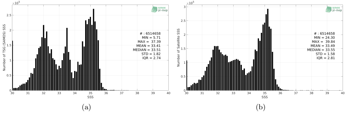
Figure 2: Histograms of SSS from TSG (SAMOS) (a) and SMOS L3 v2 - 9-Days (BEC) (b) considering all match-up pairs per bins of 0.1 over the Pacific Ocean Pi-MEP region and for the full satellite product period.
