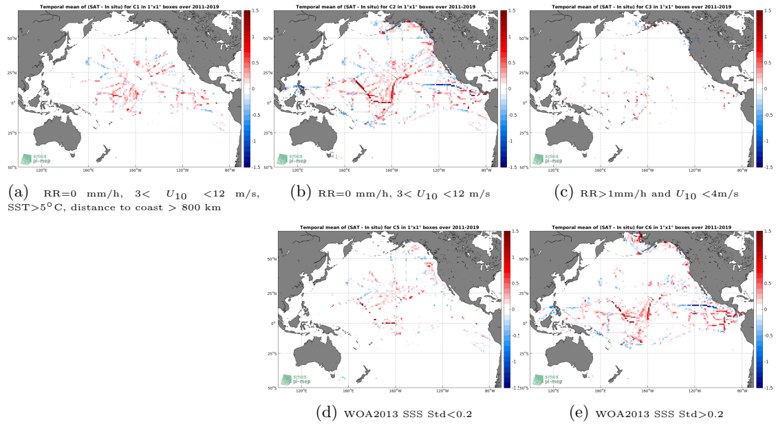
Figure 12: Temporal mean gridded over spatial boxes of size 1^\circ \times 1^\circ of \Delta SSS (SMOS L3 v2 - 9-Days (BEC) - TSG (SAMOS)) for 5 different subdatasets corresponding to:RR=0 mm/h, 3 < U_{10} < 12 m/s, SST >5^\circ\text{C} , distance to coast > 800 km (a), RR=0 mm/h, 3 < U_{10} < 12 m/s (b), RR >1 mm/h and U_{10} < 4 m/s (c), WOA2013 SSS Std <0.2 (d), WOA2013 SSS Std >0.2 (e).
