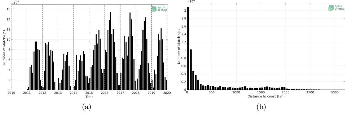
Figure 1: Number of match-ups between TSG (SAMOS) and SMOS L3 v2 - 9-Days (BEC) SSS as a function of time (a) and as function of the distance to coast (b) over the Pacific Ocean Pi-MEP region and for the full satellite product period.
