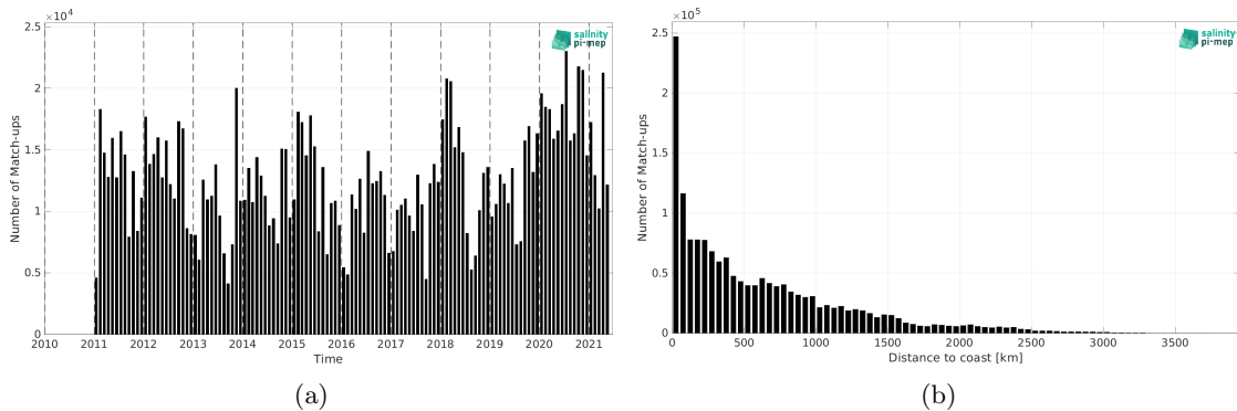
Figure 2: Number of match-ups between TSG (LEGOS-DM) and SMOS SSS L3 v2 - 9-Days (BEC) SSS as a function of time (a) and as function of the distance to coast (b) over the Pacific Ocean Pi-MEP region and for the full satellite product period.
