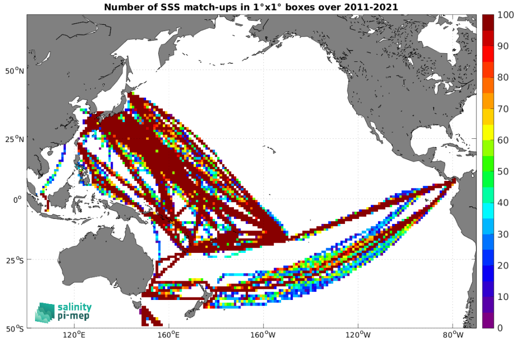
Figure 5: Number of SSS match-ups between TSG (LEGOS-DM) SSS and the SMOS SSS L3 v2 - 9-Days (BEC) SSS product for the Pacific Ocean Pi-MEP region over 1^\circ \times 1^\circ boxes and for the full satellite product period.
