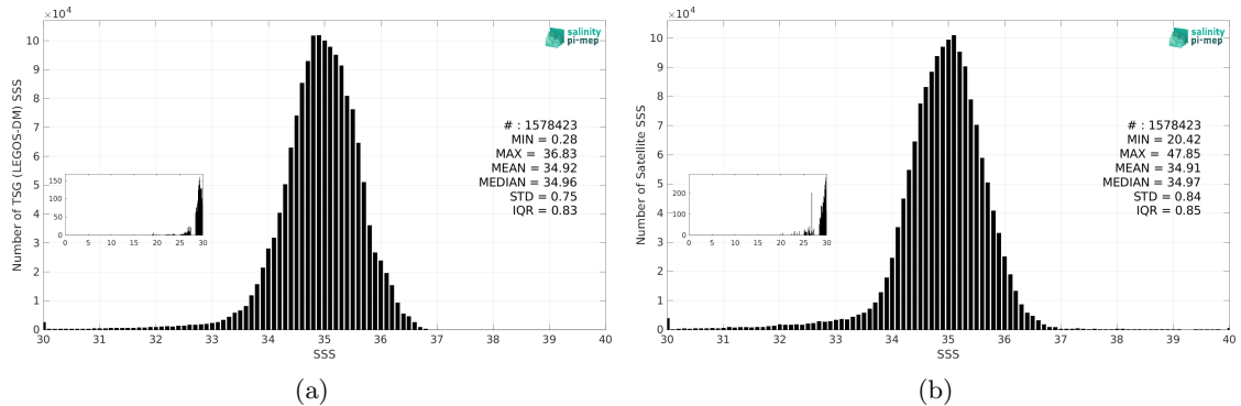
Figure 3: Histograms of SSS from TSG (LEGOS-DM) (a) and SMOS SSS L3 v2 - 9-Days (BEC) (b) considering all match-up pairs per bins of 0.1 over the Pacific Ocean Pi-MEP region and for the full satellite product period.
