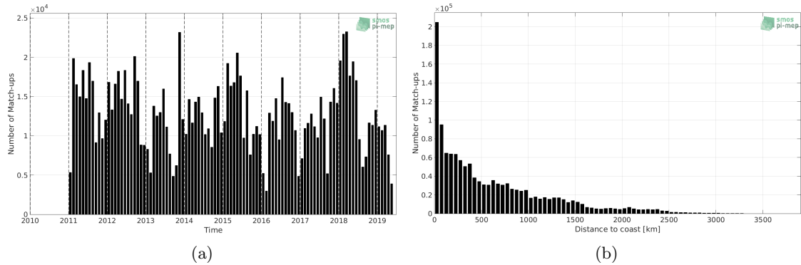
Figure 1: Number of match-ups between TSG (LEGOS-DM) and SMOS L3 v2 - 9-Days (BEC) SSS as a function of time (a) and as function of the distance to coast (b) over the Pacific Ocean Pi-MEP region and for the full satellite product period.
