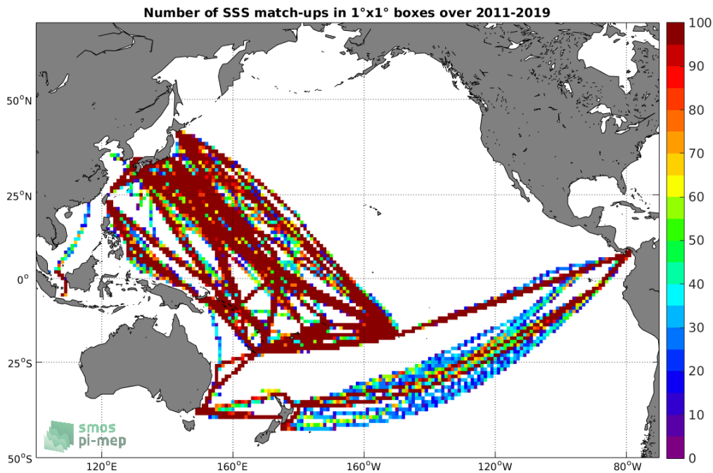
Figure 4: Number of SSS match-ups between TSG (LEGOS-DM) SSS and the SMOS L3 v2 - 9-Days (BEC) SSS product for the Pacific Ocean Pi-MEP region over 1°x1° boxes and for the full satellite product period.
