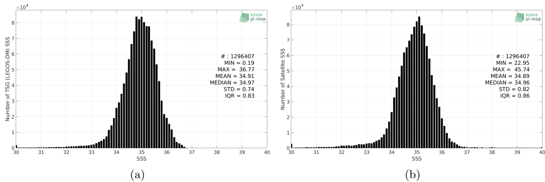
Figure 2: Histograms of SSS from TSG (LEGOS-DM) (a) and SMOS L3 v2 - 9-Days (BEC) (b) considering all match-up pairs per bins of 0.1 over the Pacific Ocean Pi-MEP region and for the full satellite product period.
