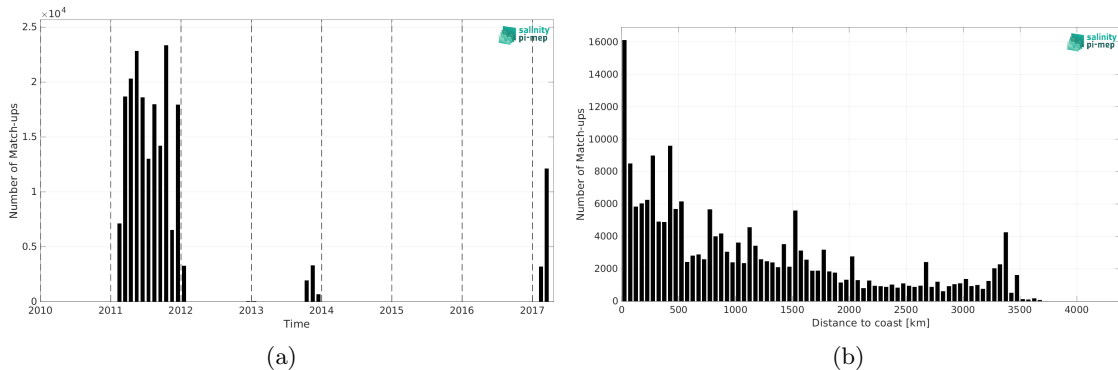
Figure 2: Number of match-ups between TSG (GOSUD-Sailing-ship) and SMOS SSS L3 v2 - 9-Days (BEC) SSS as a function of time (a) and as function of the distance to coast (b) over the Pacific Ocean Pi-MEP region and for the full satellite product period.
