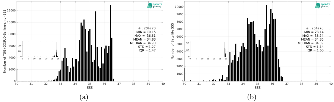
Figure 3: Histograms of SSS from TSG (GOSUD-Sailing-ship) (a) and SMOS SSS L3 v2 - 9-Days (BEC) (b) considering all match-up pairs per bins of 0.1 over the Pacific Ocean Pi-MEP region and for the full satellite product period.
