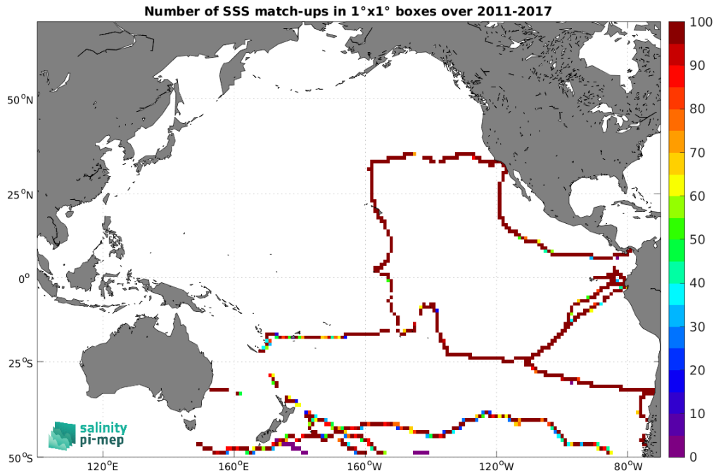
Figure 5: Number of SSS match-ups between TSG (GOSUD-Sailing-ship) SSS and the SMOS SSS L3 v2 - 9-Days (BEC) SSS product for the Pacific Ocean Pi-MEP region over 1^\circ \times 1^\circ boxes and for the full satellite product period.
