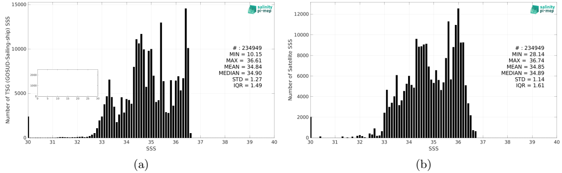
Figure 2: Histograms of SSS from TSG (GOSUD-Sailing-ship) (a) and SMOS SSS L3 v2 - 9-Days (BEC) (b) considering all match-up pairs per bins of 0.1 over the Pacific Ocean Pi-MEP region and for the full satellite product period.
