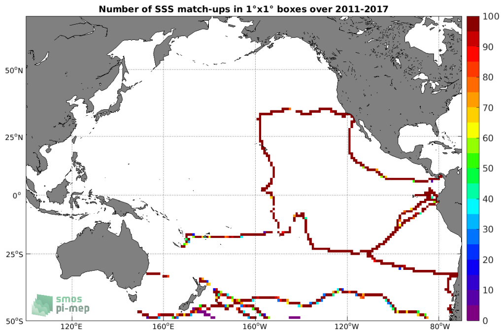
Figure 4: Number of SSS match-ups between TSG (GOSUD-Sailing-ship) SSS and the SMOS SSS L3 v2 - 9-Days (BEC) SSS product for the Pacific Ocean Pi-MEP region over 1°x1° boxes and for the full satellite product period.
