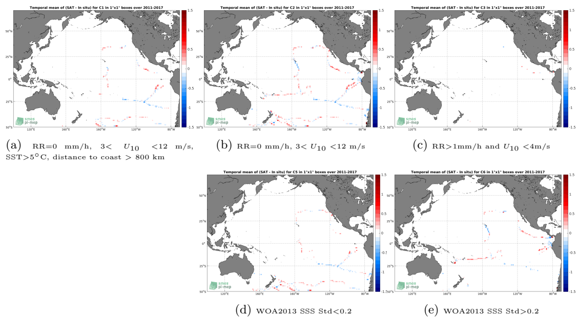
Figure 12: Temporal mean gridded over spatial boxes of size 1^\circ \times 1^\circ of \Delta SSS (SMOS L3 v2 - 9-Days (BEC) - TSG (GOSUD-Sailing-ship)) for 5 different subdatasets corresponding to: RR=0 mm/h, 3 < U_{10} < 12 m/s, SST > 5°C, distance to coast > 800 km (a), RR=0 mm/h, 3 < U_{10} < 12 m/s (b), RR > 1mm/h and U_{10} < 4 m/s (c), WOA2013 SSS Std < 0.2 (d), WOA2013 SSS Std > 0.2 (e).
