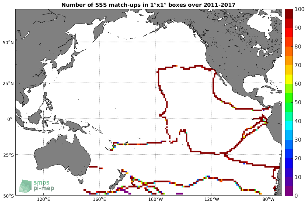
Figure 4: Number of SSS match-ups between TSG (GOSUD-Sailing-ship) SSS and the SMOS L3 v2 - 9-Days (BEC) SSS product for the Pacific Ocean Pi-MEP region over 1^\circ \times 1^\circ boxes and for the full satellite product period.
