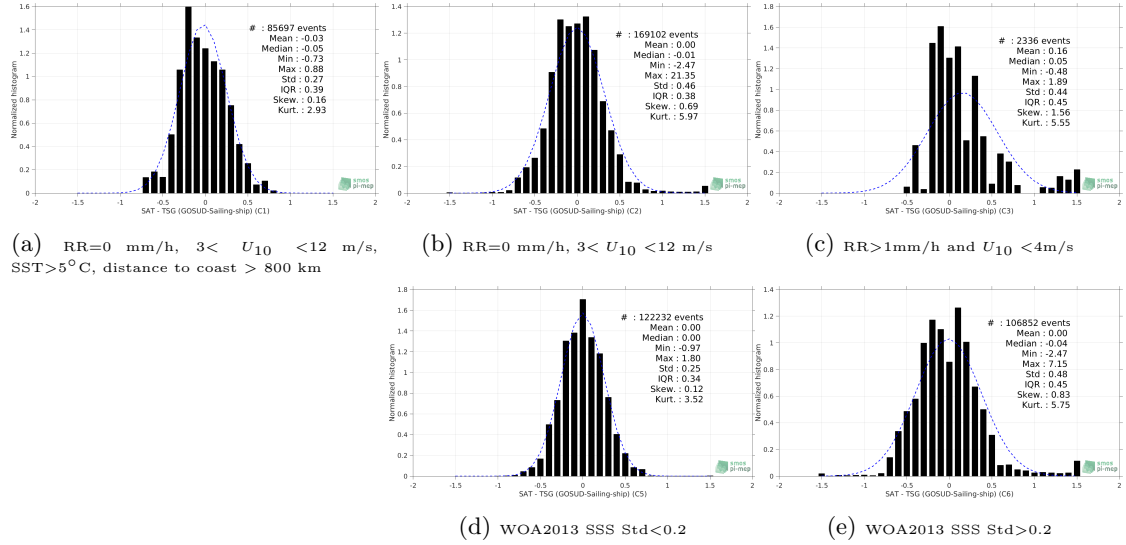
Figure 13: Normalized histogram of \Delta SSS (SMOS L3 v2 - 9-Days (BEC) - TSG (GOSUD-Sailing-ship)) for 5 different subdatasets corresponding to: RR=0 mm/h, 3 < U_{10} < 12 m/s, SST > 5°C, distance to coast > 800 km (a), RR=0 mm/h, 3 < U_{10} < 12 m/s (b), RR > 1mm/h and U_{10} < 4 m/s (c), WOA2013 SSS Std < 0.2 (d), WOA2013 SSS Std > 0.2 (e).
