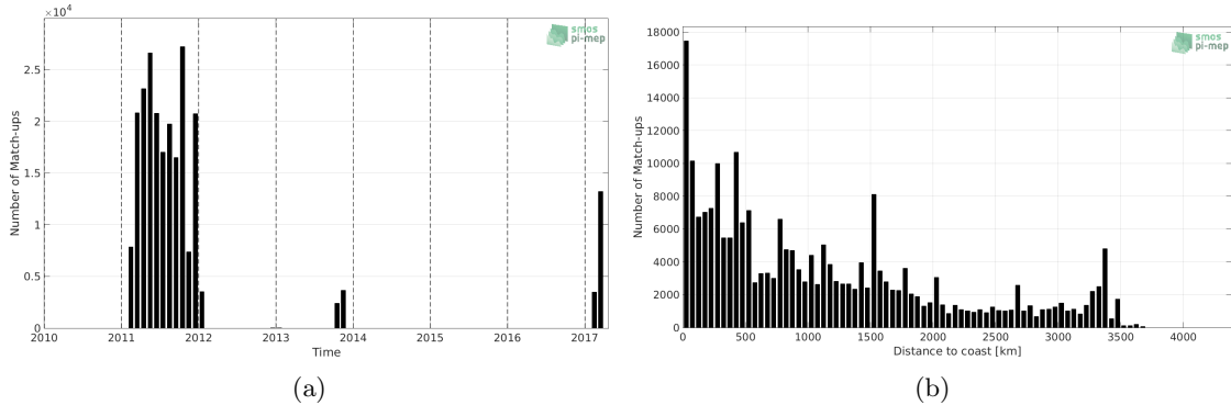
Figure 1: Number of match-ups between TSG (GOSUD-Sailing-ship) and SMOS L3 v2 - 9-Days (BEC) SSS as a function of time (a) and as function of the distance to coast (b) over the Pacific Ocean Pi-MEP region and for the full satellite product period.
