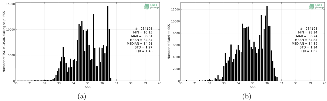
Figure 2: Histograms of SSS from TSG (GOSUD-Sailing-ship) (a) and SMOS L3 v2 - 9-Days (BEC) (b) considering all match-up pairs per bins of 0.1 over the Pacific Ocean Pi-MEP region and for the full satellite product period.
