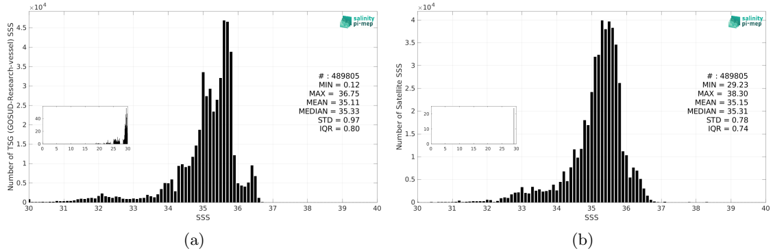
Figure 3: Histograms of SSS from TSG (GOSUD-Research-vessel) (a) and SMOS SSS L3 v2 - 9-Days (BEC) (b) considering all match-up pairs per bins of 0.1 over the Pacific Ocean Pi-MEP region and for the full satellite product period.
