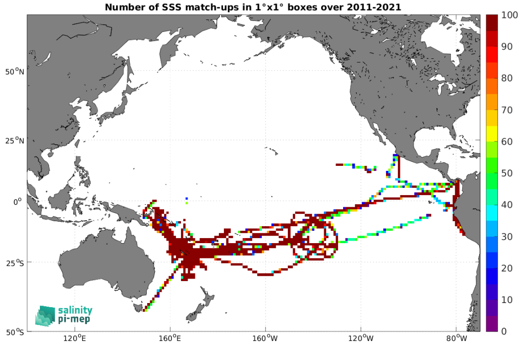
Figure 5: Number of SSS match-ups between TSG (GOSUD-Research-vessel) SSS and the SMOS SSS L3 v2 - 9-Days (BEC) SSS product for the Pacific Ocean Pi-MEP region over 1^\circ \times 1^\circ boxes and for the full satellite product period.
