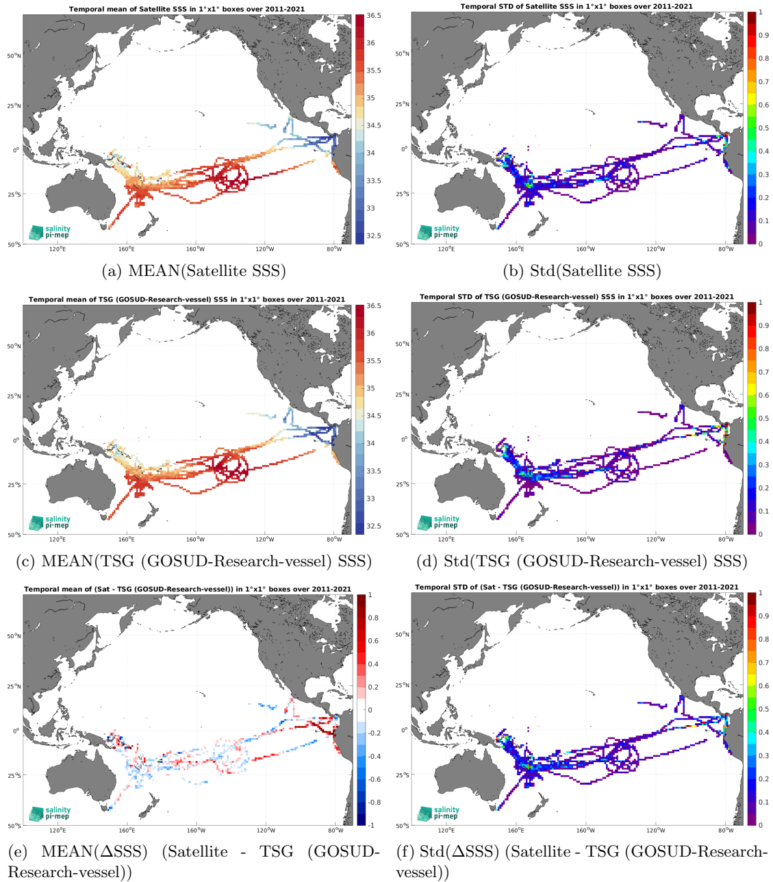
Figure 7: Temporal mean (left) and Std (right) of SSS from SMOS SSS L3 v2 - 9-Days (BEC) (top), TSG (GOSUD-Research-vessel) (middle), and of \Delta SSS (Satellite - TSG (GOSUD-Research-vessel)). Only match-up pairs are used to generate these maps.
