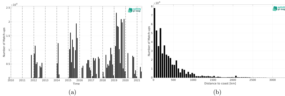
Figure 2: Number of match-ups between TSG (GOSUD-Research-vessel) and SMOS SSS L3 v2 - 9-Days (BEC) SSS as a function of time (a) and as function of the distance to coast (b) over the Pacific Ocean Pi-MEP region and for the full satellite product period.
