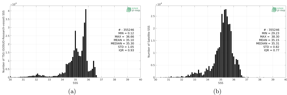
Figure 2: Histograms of SSS from TSG (GOSUD-Research-vessel) (a) and SMOS L3 v2 - 9-Days (BEC) (b) considering all match-up pairs per bins of 0.1 over the Pacific Ocean Pi-MEP region and for the full satellite product period.
