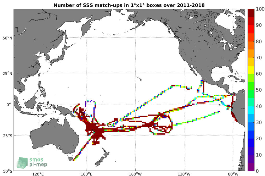
Figure 4: Number of SSS match-ups between TSG (GOSUD-Research-vessel) SSS and the SMOS L3 v2 - 9-Days (BEC) SSS product for the Pacific Ocean Pi-MEP region over 1^\circ \times 1^\circ boxes and for the full satellite product period.
