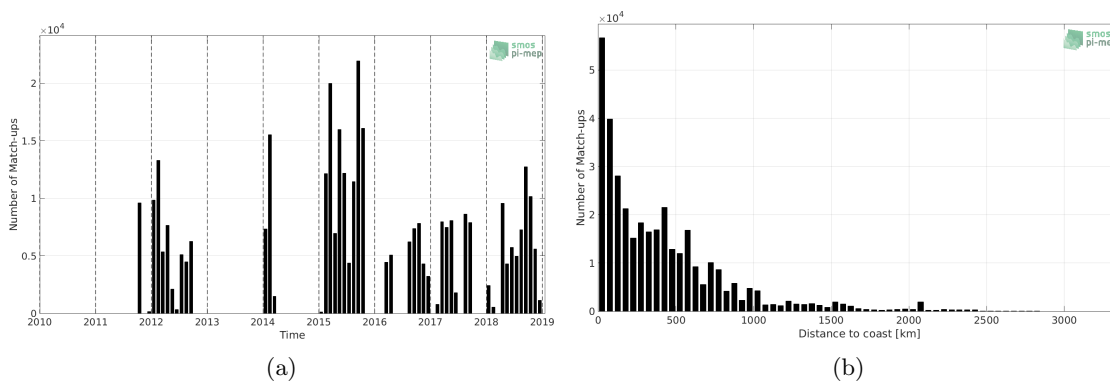
Figure 1: Number of match-ups between TSG (GOSUD-Research-vessel) and SMOS L3 v2 - 9-Days (BEC) SSS as a function of time (a) and as function of the distance to coast (b) over the Pacific Ocean Pi-MEP region and for the full satellite product period.
