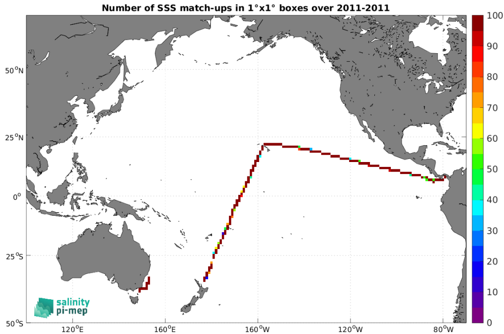
Figure 5: Number of SSS match-ups between TSG (CSIC-UTM) SSS and the SMOS SSS L3 v2 - 9-Days (BEC) SSS product for the Pacific Ocean Pi-MEP region over 1^\circ \times 1^\circ boxes and for the full satellite product period.
