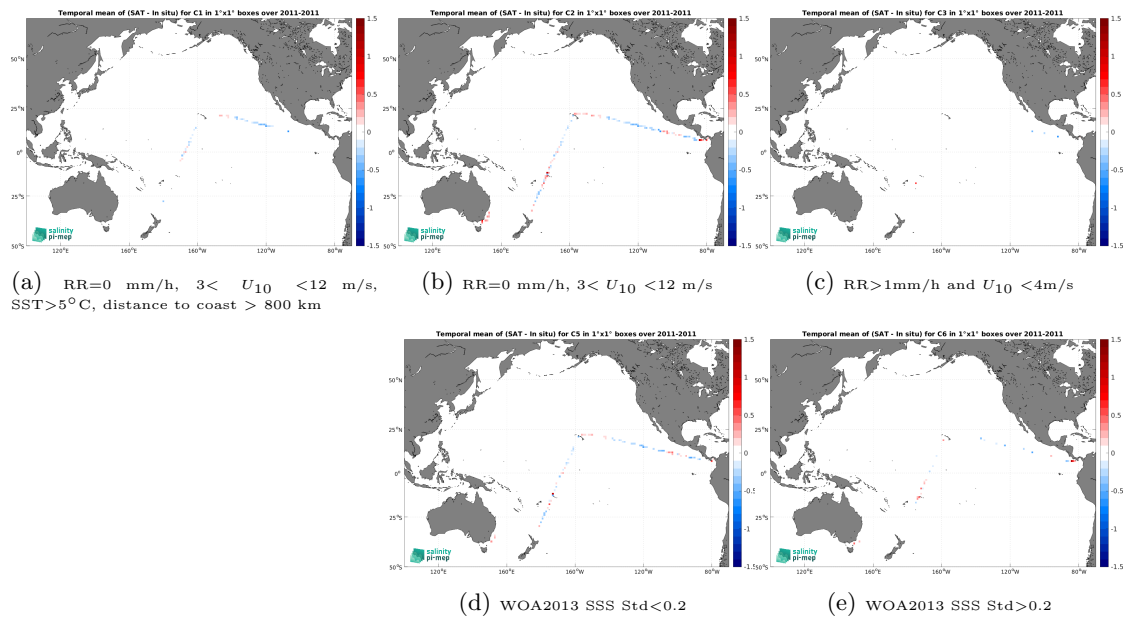
Figure 14: Temporal mean gridded over spatial boxes of size 1^\circ \times 1^\circ of \Delta SSS (SMOS SSS L3 v2 - 9-Days (BEC) - TSG (CSIC-UTM)) for 5 different subdatasets corresponding to:RR=0 mm/h, 3 < U_{10} < 12 m/s, SST >5^\circ\text{C} , distance to coast > 800 km (a), RR=0 mm/h, 3 < U_{10} < 12 m/s (b), RR >1 mm/h and U_{10} < 4 m/s (c), WOA2013 SSS Std <0.2 (d), WOA2013 SSS Std >0.2 (e).
