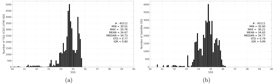
Figure 3: Histograms of SSS from TSG (CSIC-UTM) (a) and SMOS SSS L3 v2 - 9-Days (BEC) (b) considering all match-up pairs per bins of 0.1 over the Pacific Ocean Pi-MEP region and for the full satellite product period.
