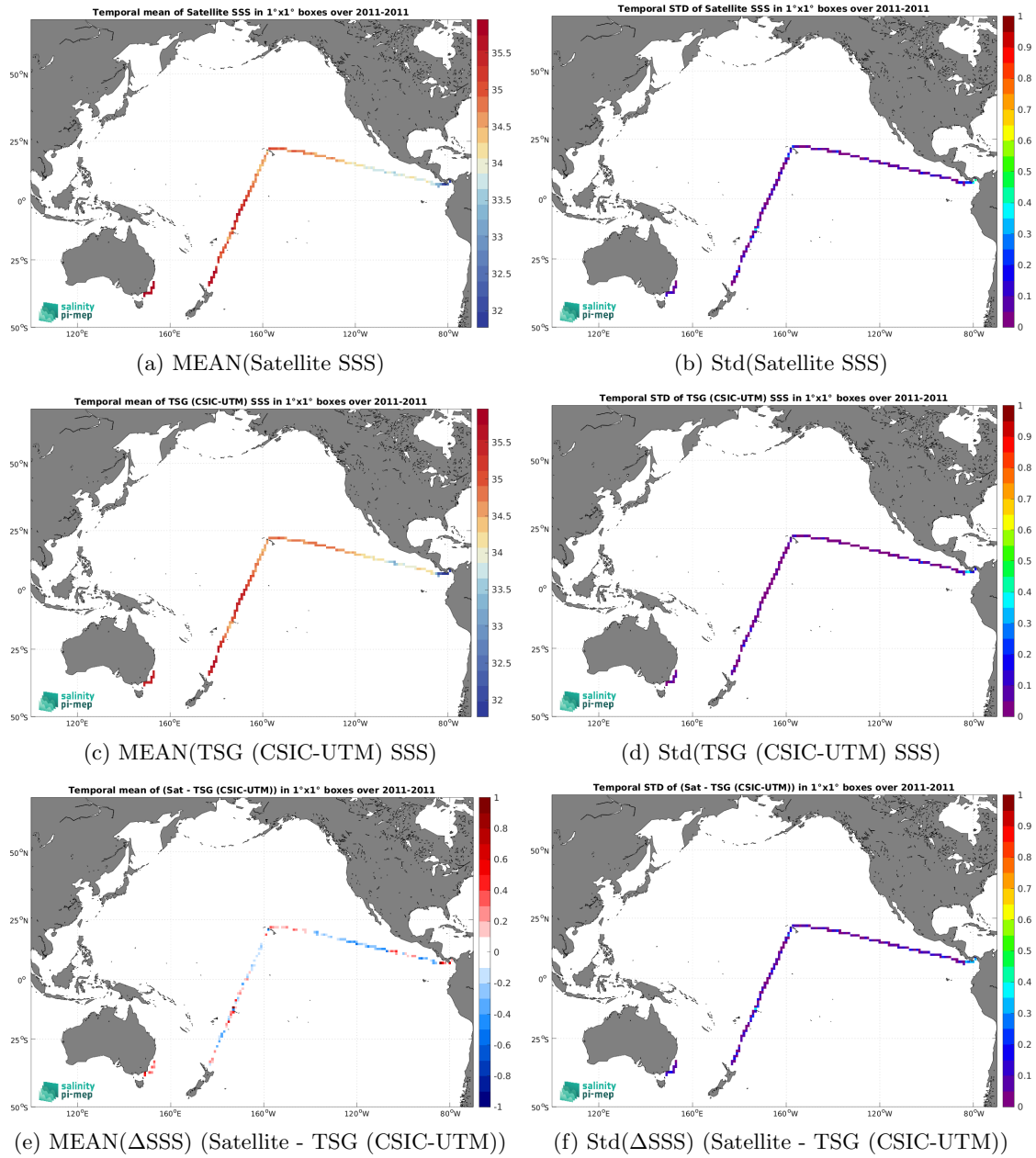
Figure 7: Temporal mean (left) and Std (right) of SSS from SMOS SSS L3 v2 - 9-Days (BEC) (top), TSG (CSIC-UTM) (middle), and of \Delta SSS (Satellite - TSG (CSIC-UTM)). Only match-up pairs are used to generate these maps.
