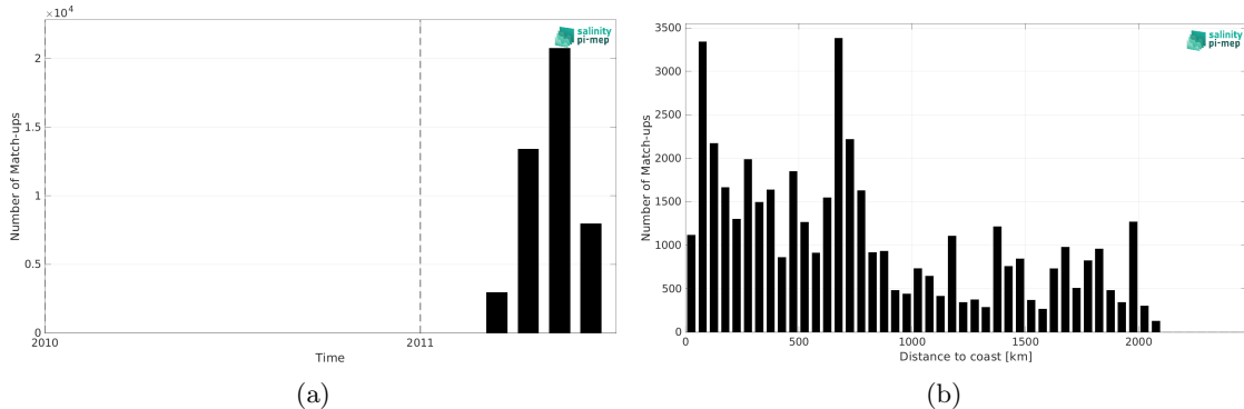
Figure 2: Number of match-ups between TSG (CSIC-UTM) and SMOS SSS L3 v2 - 9-Days (BEC) SSS as a function of time (a) and as function of the distance to coast (b) over the Pacific Ocean Pi-MEP region and for the full satellite product period.
