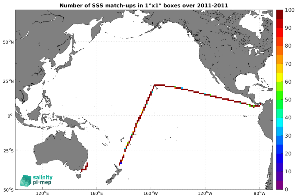
Figure 5: Number of SSS match-ups between TSG (CSIC-UTM) SSS and the SMOS SSS L3 v2 - 9-Days (BEC) SSS product for the Pacific Ocean Pi-MEP region over 1^{\circ} \times 1^{\circ} boxes and for the full satellite product period.
