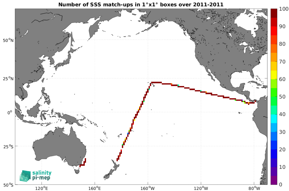
Figure 4: Number of SSS match-ups between TSG (CSIC-UTM) SSS and the SMOS SSS L3 v2 - 9-Days (BEC) SSS product for the Pacific Ocean Pi-MEP region over 1^{\circ} \times 1^{\circ} boxes and for the full satellite product period.
