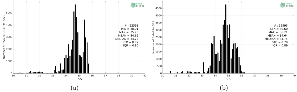
Figure 2: Histograms of SSS from TSG (CSIC-UTM) (a) and SMOS SSS L3 v2 - 9-Days (BEC) (b) considering all match-up pairs per bins of 0.1 over the Pacific Ocean Pi-MEP region and for the full satellite product period.
