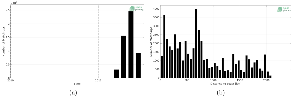
Figure 1: Number of match-ups between TSG (CSIC-UTM) and SMOS SSS L3 v2 - 9-Days (BEC) SSS as a function of time (a) and as function of the distance to coast (b) over the Pacific Ocean Pi-MEP region and for the full satellite product period.
