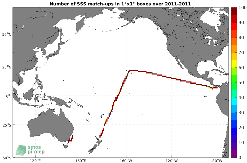
Figure 4: Number of SSS match-ups between TSG (CSIC-UTM) SSS and the SMOS SSS L3 v2 - 9-Days (BEC) SSS product for the Pacific Ocean Pi-MEP region over 1^\circ \times 1^\circ boxes and for the full satellite product period.
