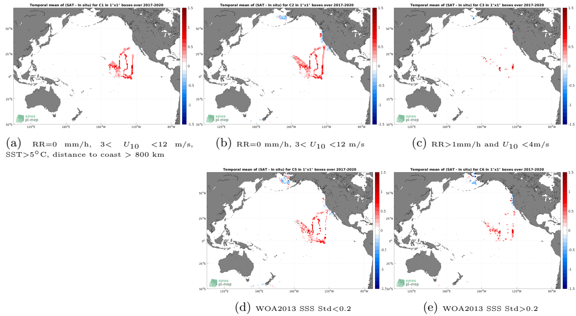
Figure 12: Temporal mean gridded over spatial boxes of size 1^\circ \times 1^\circ of \Delta SSS (SMOS SSS L3 v2 - 9-Days (BEC) - Saifdrone) for 5 different subdatasets corresponding to:RR=0 mm/h, 3 < U_{10} < 12 m/s, SST >5^\circ C, distance to coast > 800 km (a), RR=0 mm/h, 3 < U_{10} < 12 m/s (b), RR >1 mm/h and U_{10} < 4 m/s (c), WOA2013 SSS Std <0.2 (d), WOA2013 SSS Std >0.2 (e).
