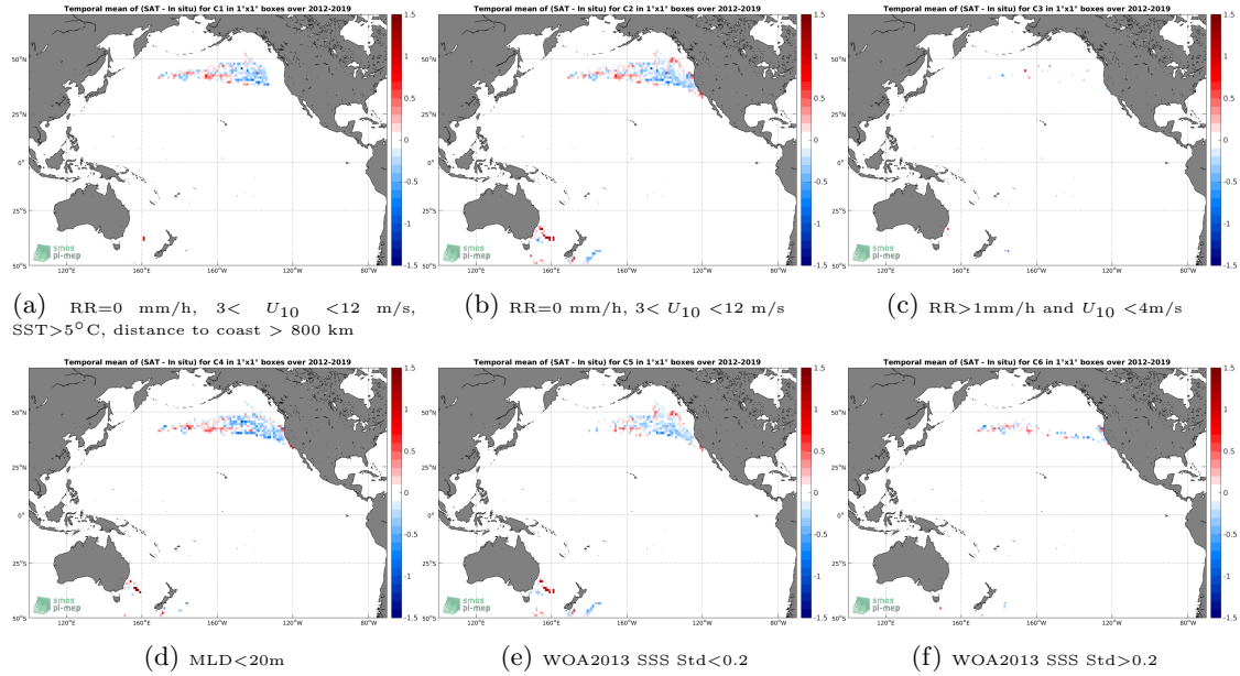
Figure 12: Temporal mean gridded over spatial boxes of size 1^\circ \times 1^\circ of \Delta SSS (SMOS SSS L3 v2 - 9-Days (BEC) - Marine mammals) for 6 different subdatasets corresponding to: RR=0 mm/h, 3 < U_{10} < 12 m/s, SST > 5^\circ C , distance to coast > 800 km (a), RR=0 mm/h, 3 < U_{10} < 12 m/s (b), RR > 1 mm/h and U_{10} < 4 m/s (c), MLD < 20 m (d), WOA2013 SSS Std < 0.2 (e), WOA2013 SSS Std > 0.2 (f).
