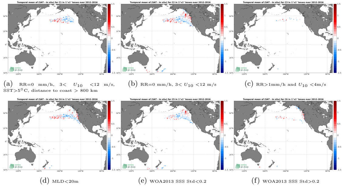
Figure 12: Temporal mean gridded over spatial boxes of size 1^\circ \times 1^\circ of \Delta SSS (SMOS SSS L3 v2 - 9-Days (BEC) - Sea mammals) for 6 different subdatasets corresponding to: RR=0 mm/h, 3 < U_{10} < 12 m/s, SST > 5^\circ C , distance to coast > 800 km (a), RR=0 mm/h, 3 < U_{10} < 12 m/s (b), RR > 1 mm/h and U_{10} < 4 m/s (c), MLD < 20 m (d), WOA2013 SSS Std < 0.2 (e), WOA2013 SSS Std > 0.2 (f).
