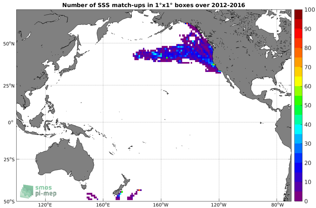
Figure 4: Number of SSS match-ups between Sea mammals SSS and the SMOS SSS L3 v2 - 9-Days (BEC) SSS product for the Pacific Ocean Pi-MEP region over 1°x1° boxes and for the full satellite product period.
