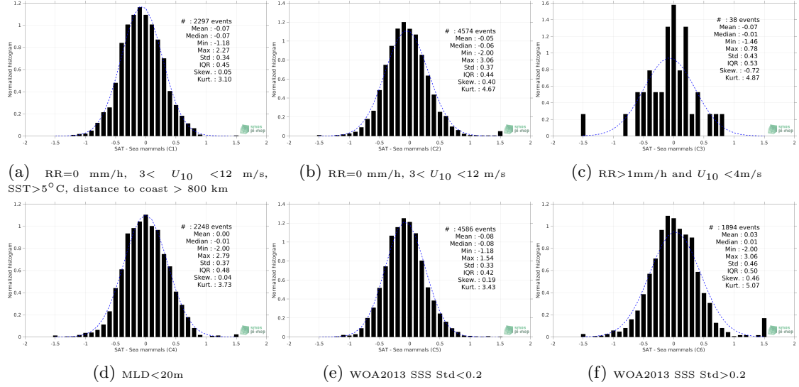
Figure 13: Normalized histogram of \Delta\text{SSS} (SMOS SSS L3 v2 - 9-Days (BEC) - Sea mammals) for 6 different subdatasets corresponding to: RR=0 mm/h, 3 < U_{10} < 12 m/s, SST>5°C, distance to coast > 800 km (a), RR=0 mm/h, 3 < U_{10} < 12 m/s (b), RR>1mm/h and U_{10} < 4 m/s (c), MLD<20m (d), WOA2013 SSS Std<0.2 (e), WOA2013 SSS Std>0.2 (f).
