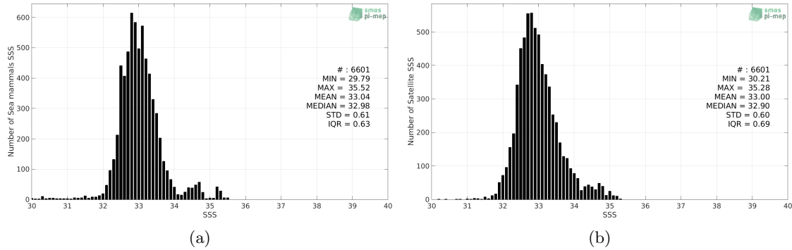
Figure 2: Histograms of SSS from Sea mammals (a) and SMOS SSS L3 v2 - 9-Days (BEC) (b) considering all match-up pairs per bins of 0.1 over the Pacific Ocean Pi-MEP region and for the full satellite product period.
