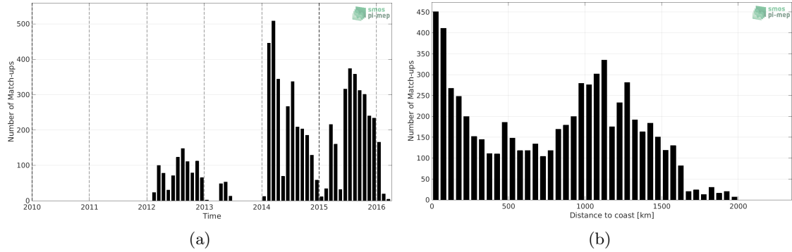
Figure 1: Number of match-ups between Sea mammals and SMOS SSS L3 v2 - 9-Days (BEC) SSS as a function of time (a) and as function of the distance to coast (b) over the Pacific Ocean Pi-MEP region and for the full satellite product period.
