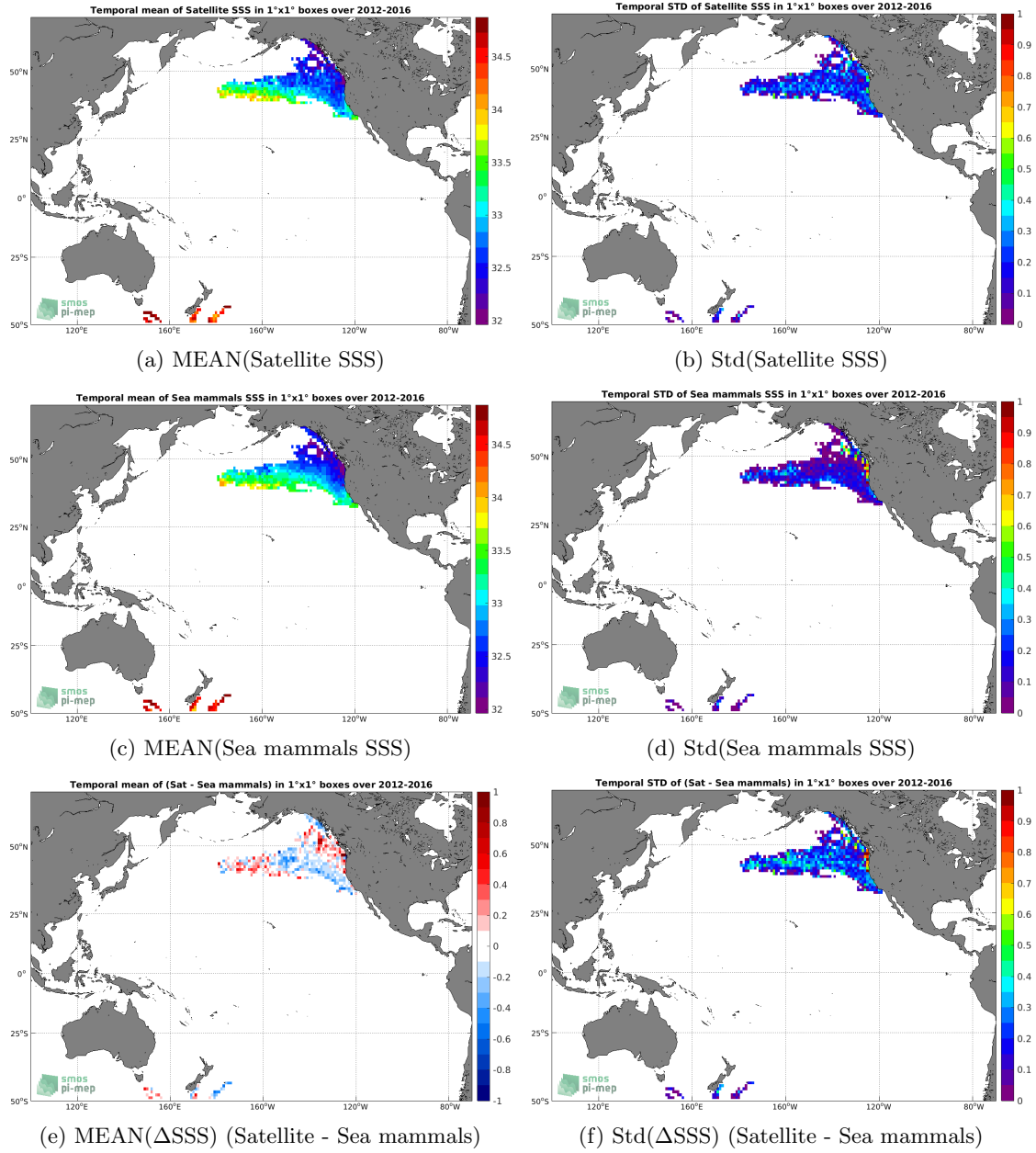
Figure 6: Temporal mean (left) and Std (right) of SSS from SMOS SSS L3 v2 - 9-Days (BEC) (top), Sea mammals (middle), and of \Delta SSS (Satellite - Sea mammals). Only match-up pairs are used to generate these maps.
