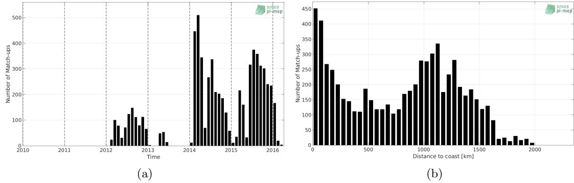
Figure 1: Number of match-ups between Sea mammals and SMOS L3 v2 - 9-Days (BEC) SSS as a function of time (a) and as function of the distance to coast (b) over the Pacific Ocean Pi-MEP region and for the full satellite product period.
