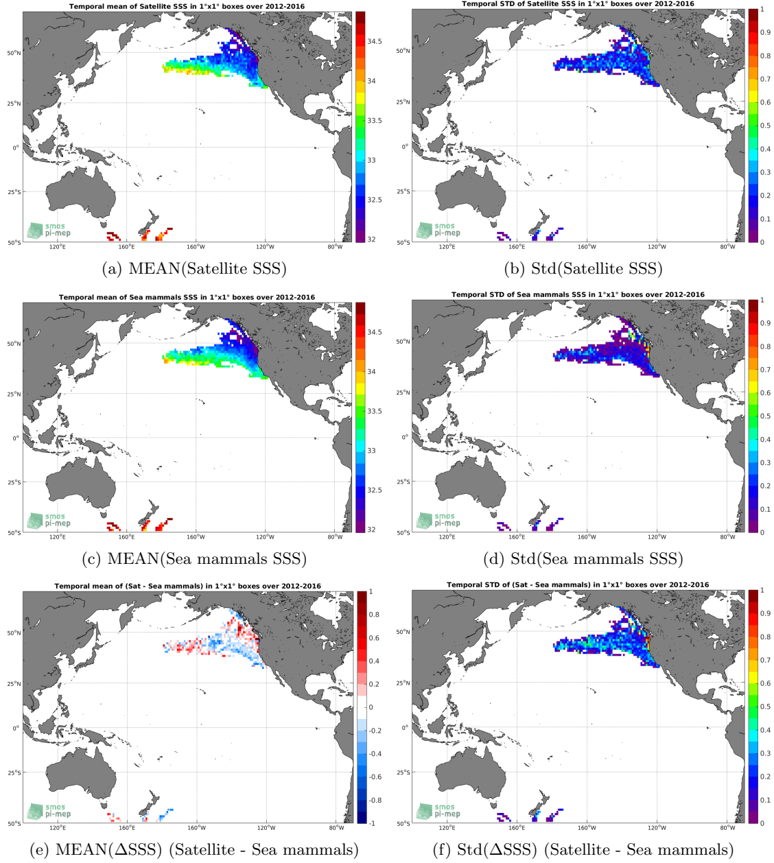
Figure 6: Temporal mean (left) and Std (right) of SSS from SMOS L3 v2 - 9-Days (BEC) (top), Sea mammals (middle), and of \Delta SSS (Satellite - Sea mammals). Only match-up pairs are used to generate these maps.
