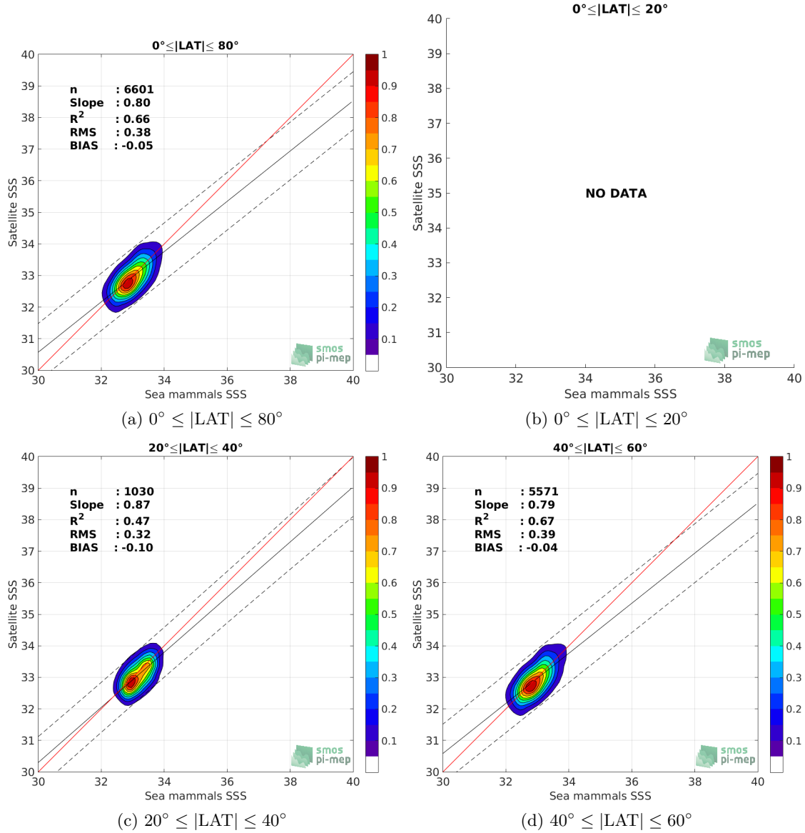
Figure 9: Contour maps of the concentration of SMOS L3 v2 - 9-Days (BEC) SSS (y-axis) versus Sea mammals SSS (x-axis) at match-up pairs for different latitude bands. For each plot, the red line shows x=y . The black thin and dashed lines indicate a linear fit through the data cloud and the \pm 95\% confidence levels, respectively. The number match-up pairs n , the slope and R^2 coefficient of the linear fit, the root mean square (RMS) and the mean bias between satellite and in situ data are indicated for each latitude band in each plots.
