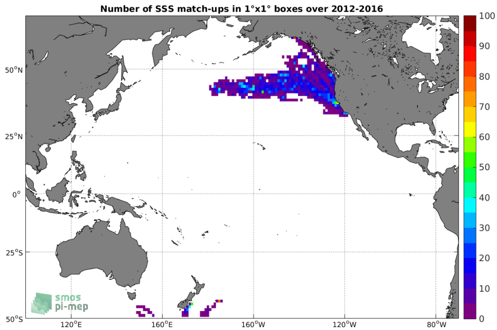
Figure 4: Number of SSS match-ups between Sea mammals SSS and the SMOS L3 v2 - 9-Days (BEC) SSS product for the Pacific Ocean Pi-MEP region over 1°x1° boxes and for the full satellite product period.
