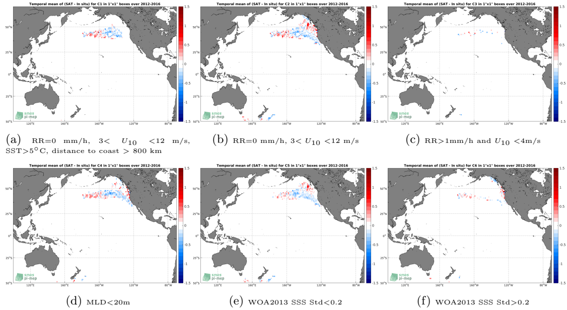
Figure 12: Temporal mean gridded over spatial boxes of size 1^\circ \times 1^\circ of \Delta SSS (SMOS L3 v2 - 9-Days (BEC) - Sea mammals) for 6 different subdatasets corresponding to: RR=0 mm/h, 3 < U_{10} < 12 m/s, SST > 5^\circ C , distance to coast > 800 km (a), RR=0 mm/h, 3 < U_{10} < 12 m/s (b), RR > 1 mm/h and U_{10} < 4 m/s (c), MLD < 20 m (d), WOA2013 SSS Std < 0.2 (e), WOA2013 SSS Std > 0.2 (f).
