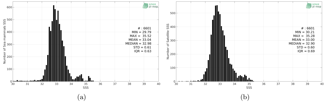
Figure 2: Histograms of SSS from Sea mammals (a) and SMOS L3 v2 - 9-Days (BEC) (b) considering all match-up pairs per bins of 0.1 over the Pacific Ocean Pi-MEP region and for the full satellite product period.
