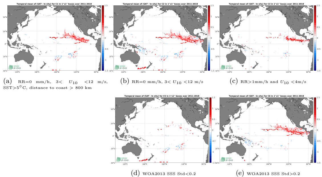
Figure 11: Temporal mean gridded over spatial boxes of size 1^\circ \times 1^\circ of \Delta SSS (SMOS SSS L3 v2 - 9-Days (BEC) - Surface drifters) for 5 different subdatasets corresponding to: RR=0 mm/h, 3 < U_{10} < 12 m/s, SST > 5°C, distance to coast > 800 km (a), RR=0 mm/h, 3 < U_{10} < 12 m/s (b), RR > 1mm/h and U_{10} < 4 m/s (c), WOA2013 SSS Std < 0.2 (d), WOA2013 SSS Std > 0.2 (e).
