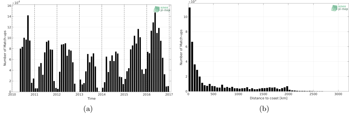
Figure 1: Number of match-ups between TSG-SAMOS and SMOS-L3-BEC-OA-V1-9DAYS-0.25DEG SSS as a function of time (a) and as function of the distance to coast (b) over the Pacific Ocean Pi-MEP region and for the full satellite product period.
