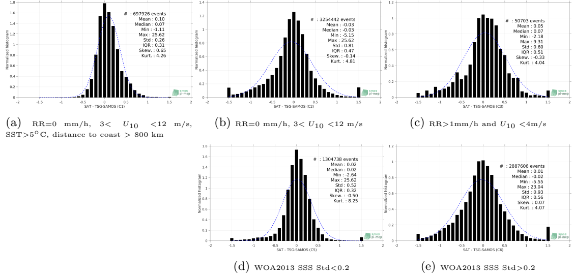
Figure 13: Normalized histogram of \Delta SSS (SMOS-L3-BEC-OA-V1-9DAYS-0.25DEG - TSG-SAMOS) for 5 different subdatasets corresponding to: RR=0 mm/h, 3 < U_{10} < 12 m/s, SST>5°C, distance to coast > 800 km (a), RR=0 mm/h, 3 < U_{10} < 12 m/s (b), RR>1mm/h and U_{10} < 4 m/s (c), WOA2013 SSS Std<0.2 (d), WOA2013 SSS Std>0.2 (e).
