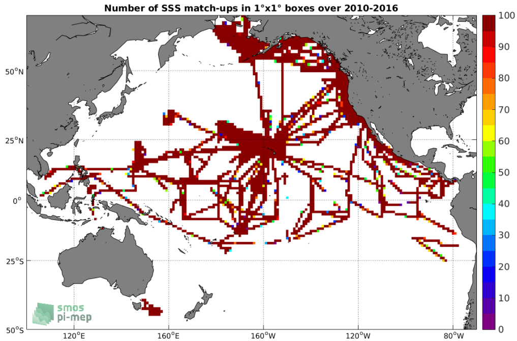
Figure 4: Number of SSS match-ups between TSG-SAMOS SSS and the SMOS-L3-BEC-OA-V1-9DAYS-0.25DEG SSS product for the Pacific Ocean Pi-MEP region over 1°x1° boxes and for the full satellite product period.
