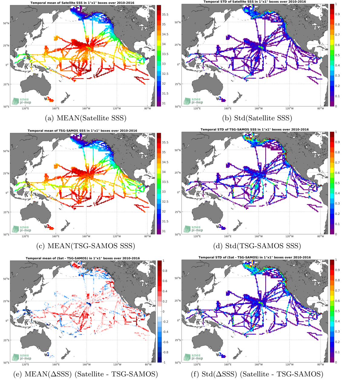
Figure 6: Temporal mean (left) and Std (right) of SSS from SMOS-L3-BEC-OA-V1-9DAYS-0.25DEG (top), TSG-SAMOS (middle), and of \Delta SSS (Satellite - TSG-SAMOS). Only match-up pairs are used to generate these maps.
