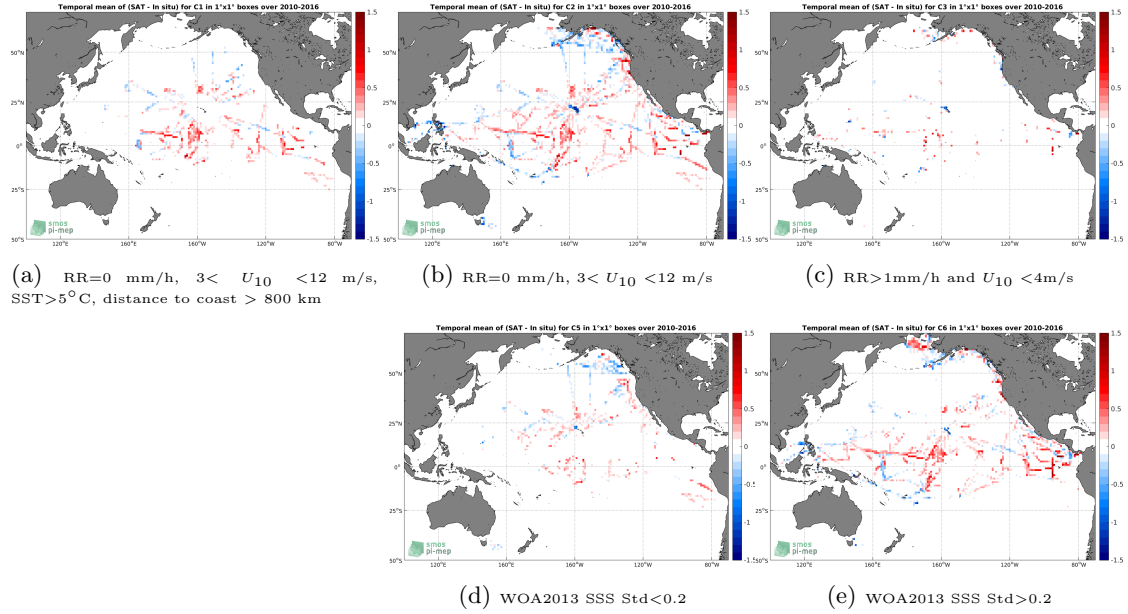
Figure 12: Temporal mean gridded over spatial boxes of size 1^\circ \times 1^\circ of \Delta SSS (SMOS-L3-BEC-OA-V1-9DAYS-0.25DEG - TSG-SAMOS) for 5 different subdatasets corresponding to: RR=0 mm/h, 3 < U_{10} < 12 m/s, SST > 5^\circ C , distance to coast > 800 km (a), RR=0 mm/h, 3 < U_{10} < 12 m/s (b), RR > 1 mm/h and U_{10} < 4 m/s (c), WOA2013 SSS Std < 0.2 (d), WOA2013 SSS Std > 0.2 (e).
