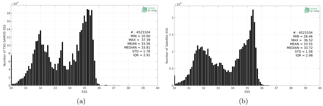
Figure 2: Histograms of SSS from TSG-SAMOS (a) and SMOS-L3-BEC-OA-V1-9DAYS-0.25DEG (b) considering all match-up pairs per bins of 0.1 over the Pacific Ocean Pi-MEP region and for the full satellite product period.
