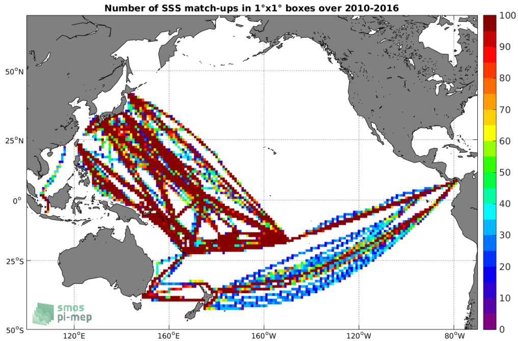
Figure 4: Number of SSS match-ups between TSG-LEGOS-DM SSS and the SMOS-L3-BEC-OA-V1-9DAYS-0.25DEG SSS product for the Pacific Ocean Pi-MEP region over 1^\circ \times 1^\circ boxes and for the full satellite product period.
