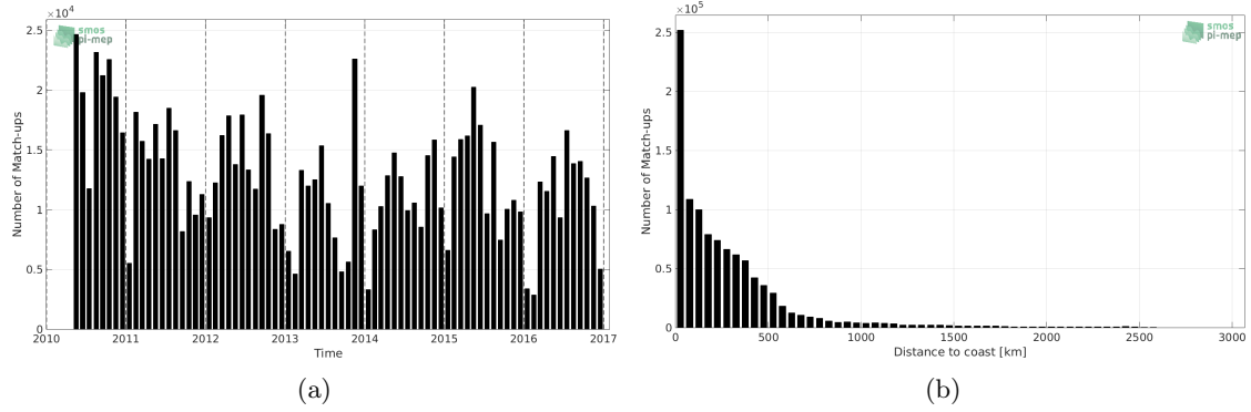
Figure 1: Number of match-ups between TSG-LEGOS-DM and SMOS-L3-BEC-OA-V1-9DAYS-0.25DEG SSS as a function of time (a) and as function of the distance to coast (b) over the Pacific Ocean Pi-MEP region and for the full satellite product period.
