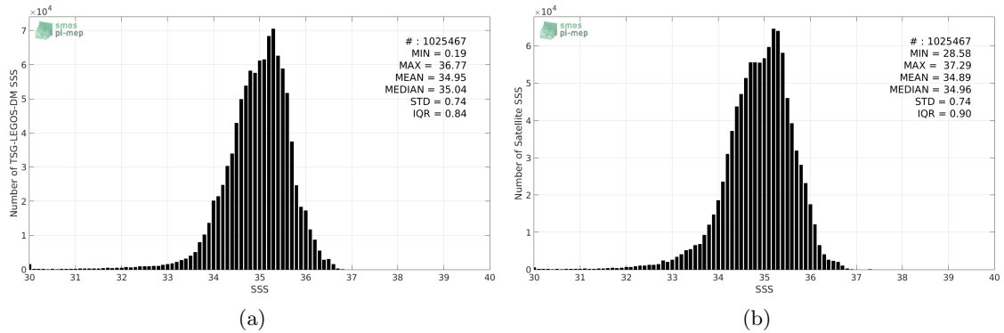
Figure 2: Histograms of SSS from TSG-LEGOS-DM (a) and SMOS-L3-BEC-OA-V1-9DAYS-0.25DEG (b) considering all match-up pairs per bins of 0.1 over the Pacific Ocean Pi-MEP region and for the full satellite product period.
