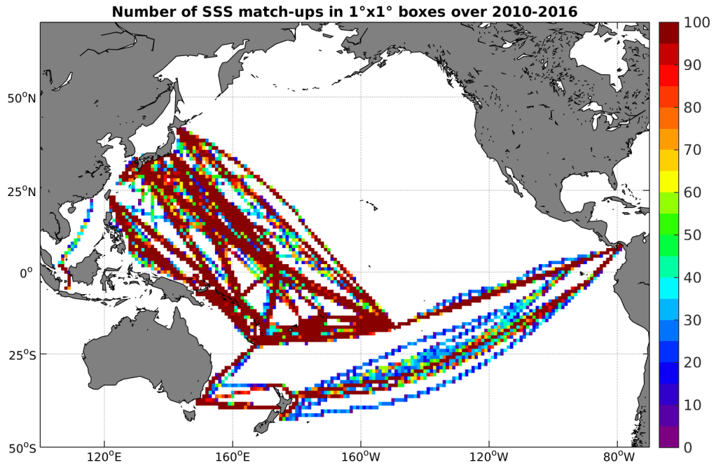
Figure 4: Number of SSS match-ups between TSG-LEGOS-DM SSS and the SMOS-L3-BEC-OA-V1-9DAYS-0.25DEG SSS product for the Pacific Ocean Pi-MEP region over 1^\circ \times 1^\circ boxes and for the full satellite product period.
