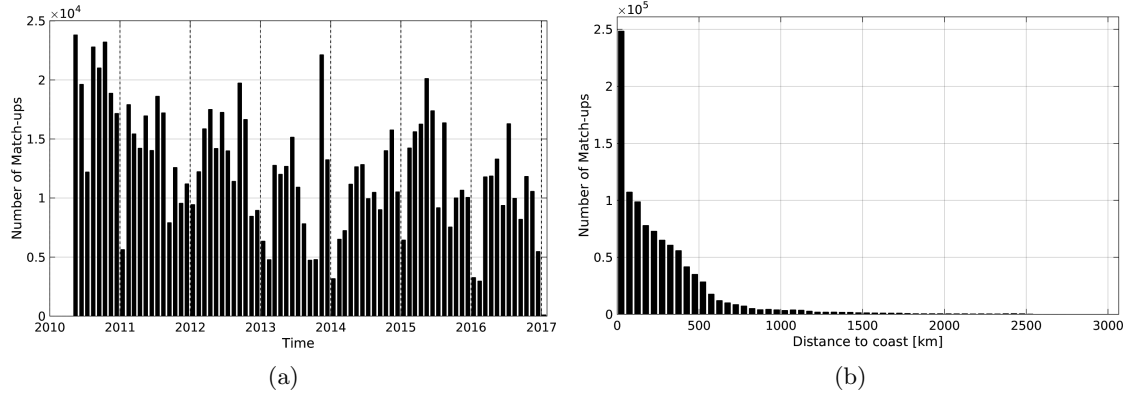
Figure 1: Number of match-ups between TSG-LEGOS-DM and SMOS-L3-BEC-OA-V1-9DAYS-0.25DEG SSS as a function of time (a) and as function of the distance to coast (b) over the Pacific Ocean Pi-MEP region and for the full satellite product period.
