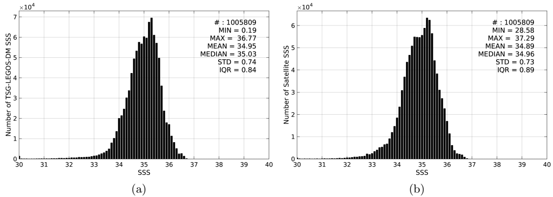
Figure 2: Histograms of SSS from TSG-LEGOS-DM (a) and SMOS-L3-BEC-OA-V1-9DAYS-0.25DEG (b) considering all match-up pairs per bins of 0.1 over the Pacific Ocean Pi-MEP region and for the full satellite product period.
