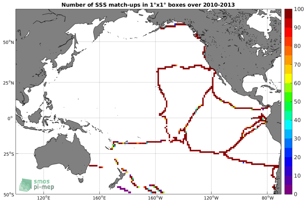
Figure 4: Number of SSS match-ups between TSG-GOSUD-Sailing-ship SSS and the SMOS-L3-BEC-OA-V1-9DAYS-0.25DEG SSS product for the Pacific Ocean Pi-MEP region over 1^\circ \times 1^\circ boxes and for the full satellite product period.
