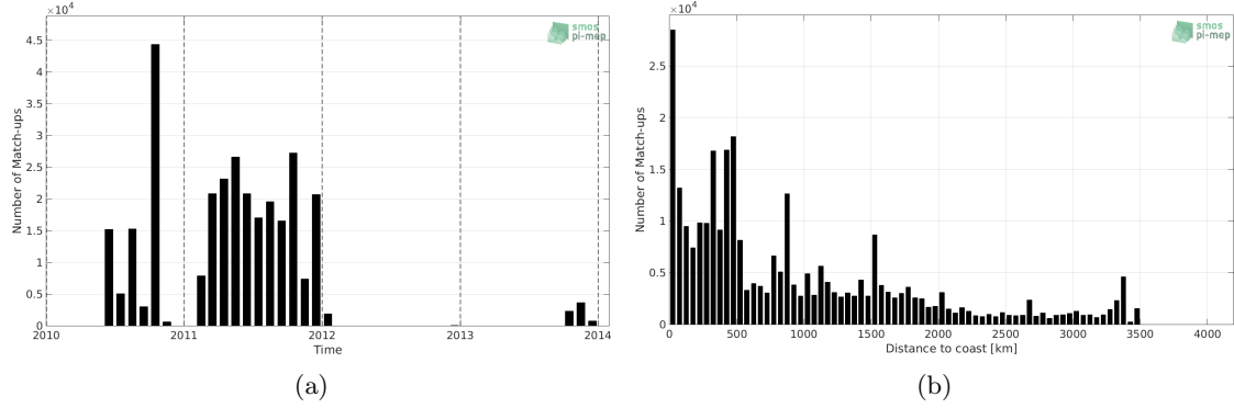
Figure 1: Number of match-ups between TSG-GOSUD-Sailing-ship and SMOS-L3-BEC-OA-V1-9DAYS-0.25DEG SSS as a function of time (a) and as function of the distance to coast (b) over the Pacific Ocean Pi-MEP region and for the full satellite product period.
