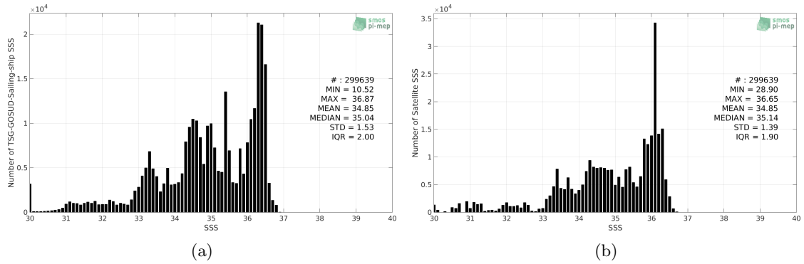
Figure 2: Histograms of SSS from TSG-GOSUD-Sailing-ship (a) and SMOS-L3-BEC-OA-V1-9DAYS-0.25DEG (b) considering all match-up pairs per bins of 0.1 over the Pacific Ocean Pi-MEP region and for the full satellite product period.
