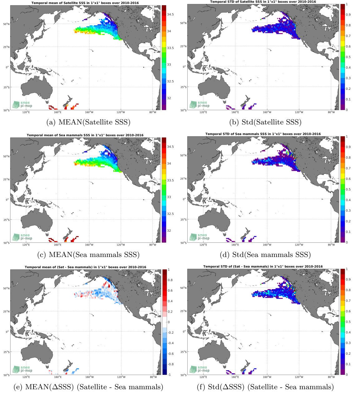
Figure 6: Temporal mean (left) and Std (right) of SSS from SMOS-L3-BEC-OA-V1-9DAYS-0.25DEG (top), Sea mammals (middle), and of \Delta SSS (Satellite - Sea mammals). Only match-up pairs are used to generate these maps.
