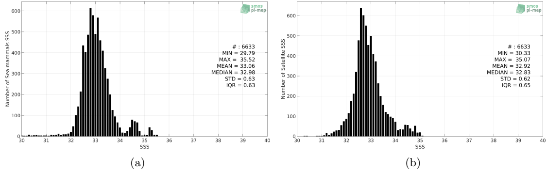
Figure 2: Histograms of SSS from Sea mammals (a) and SMOS-L3-BEC-OA-V1-9DAYS-0.25DEG (b) considering all match-up pairs per bins of 0.1 over the Pacific Ocean Pi-MEP region and for the full satellite product period.
