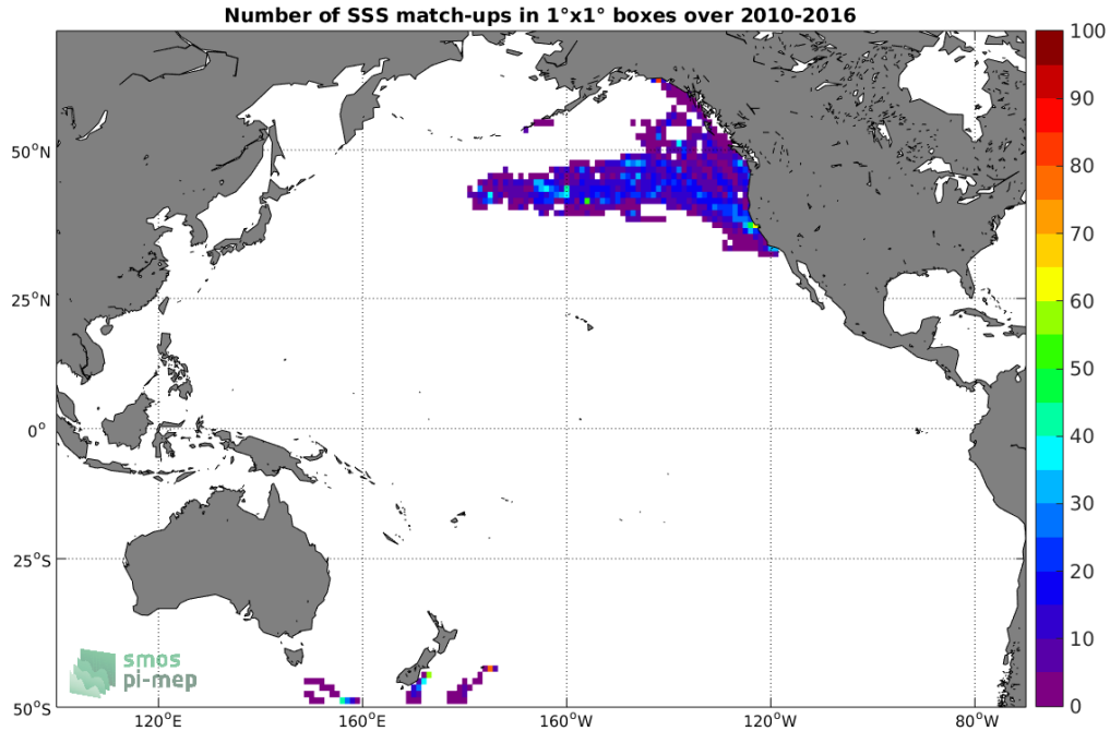
Figure 4: Number of SSS match-ups between Sea mammals SSS and the SMOS-L3-BEC-OA-V1-9DAYS-0.25DEG SSS product for the Pacific Ocean Pi-MEP region over 1°x1° boxes and for the full satellite product period.
