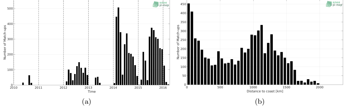
Figure 1: Number of match-ups between Sea mammals and SMOS-L3-BEC-OA-V1-9DAYS-0.25DEG SSS as a function of time (a) and as function of the distance to coast (b) over the Pacific Ocean Pi-MEP region and for the full satellite product period.
