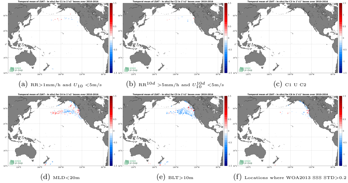
Figure 12: Temporal mean gridded over spatial boxes of size 1^\circ \times 1^\circ of \Delta\text{SSS} (SMOS-L3-BEC-OA-V1-9DAYS-0.25DEG - Sea mammals) for 6 different subdatasets corresponding to: \text{RR} > 1\text{mm/h} and U_{10} < 5\text{m/s} (a), \text{RR}^{10d} > 5\text{mm/h} and U_{10}^{10d} < 5\text{m/s} (b), \text{C1} \cup \text{C2} (c), \text{MLD} < 20\text{m} (d), \text{BLT} > 10\text{m} (e), Locations where WOA2013 SSS STD > 0.2 (f).
