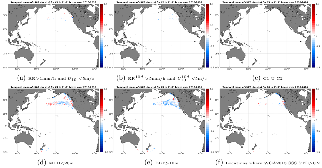
Figure 12: Temporal mean gridded over spatial boxes of size 1^\circ \times 1^\circ of \Delta SSS (SMOS-L3-BEC-OA-V1-9DAYS-0.25DEG - Sea mammals) for 6 different subdatasets corresponding to: RR > 1\text{mm/h} and U_{10} < 5\text{m/s} (a), RR^{10d} > 5\text{mm/h} and U_{10}^{10d} < 5\text{m/s} (b), C1 U C2 (c), MLD < 20\text{m} (d), BLT > 10\text{m} (e), Locations where WOA2013 SSS STD > 0.2 (f).
