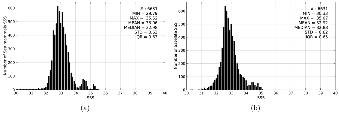
Figure 2: Histograms of SSS from Sea mammals (a) and SMOS-L3-BEC-OA-V1-9DAYS-0.25DEG (b) considering all match-up pairs per bins of 0.1 over the Pacific Ocean Pi-MEP region and for the full satellite product period.
