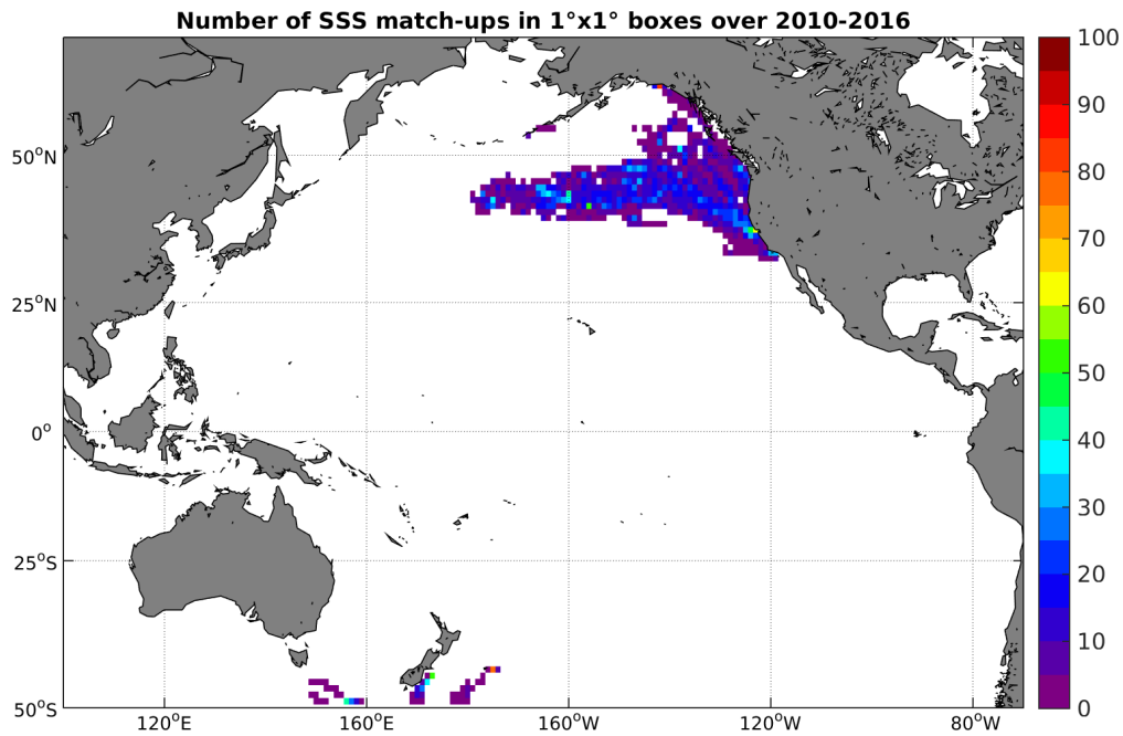
Figure 4: Number of SSS match-ups between Sea mammals SSS and the SMOS-L3-BEC-OA-V1-9DAYS-0.25DEG SSS product for the Pacific Ocean Pi-MEP region over 1^\circ \times 1^\circ boxes and for the full satellite product period.
