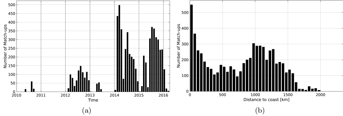
Figure 1: Number of match-ups between Sea mammals and SMOS-L3-BEC-OA-V1-9DAYS-0.25DEG SSS as a function of time (a) and as function of the distance to coast (b) over the Pacific Ocean Pi-MEP region and for the full satellite product period.
