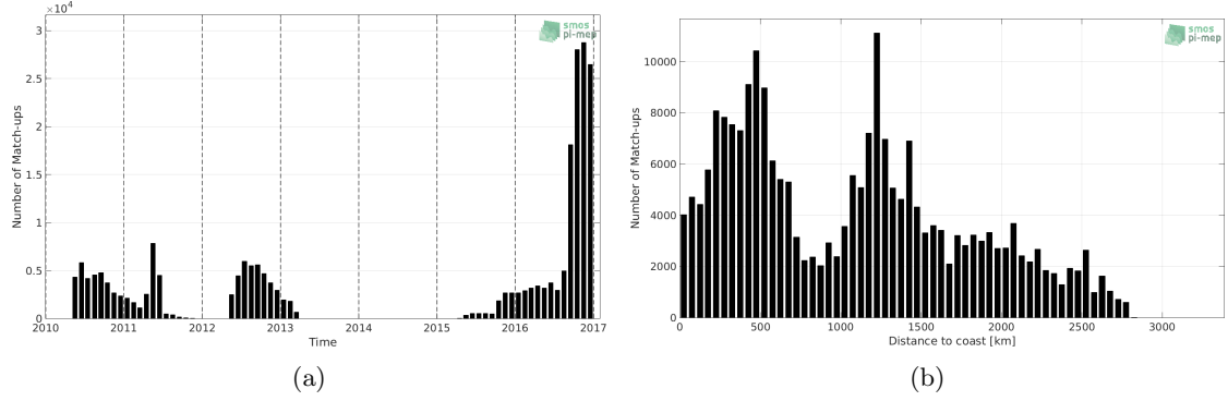
Figure 1: Number of match-ups between Surface drifters and SMOS-L3-BEC-OA-V1-9DAYS-0.25DEG SSS as a function of time (a) and as function of the distance to coast (b) over the Pacific Ocean Pi-MEP region and for the full satellite product period.
